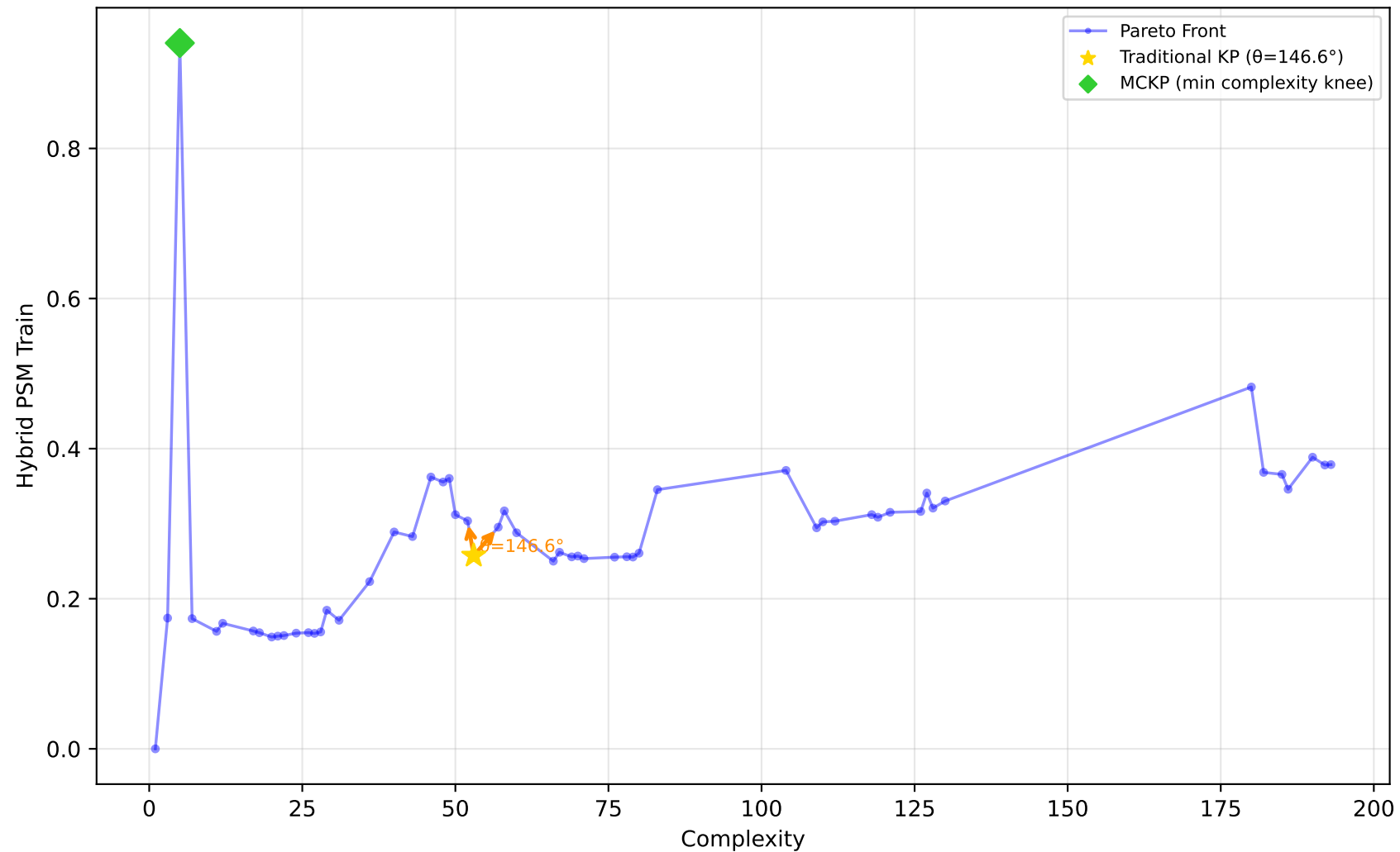
712_chscase_geyser1 - Run 25 - MVP - Hybrid PSM Train \lambda_1=1.00, \lambda_2=1.00, \lambda_3=1.00 | Difficulty: 0.84 | Method: hmr
