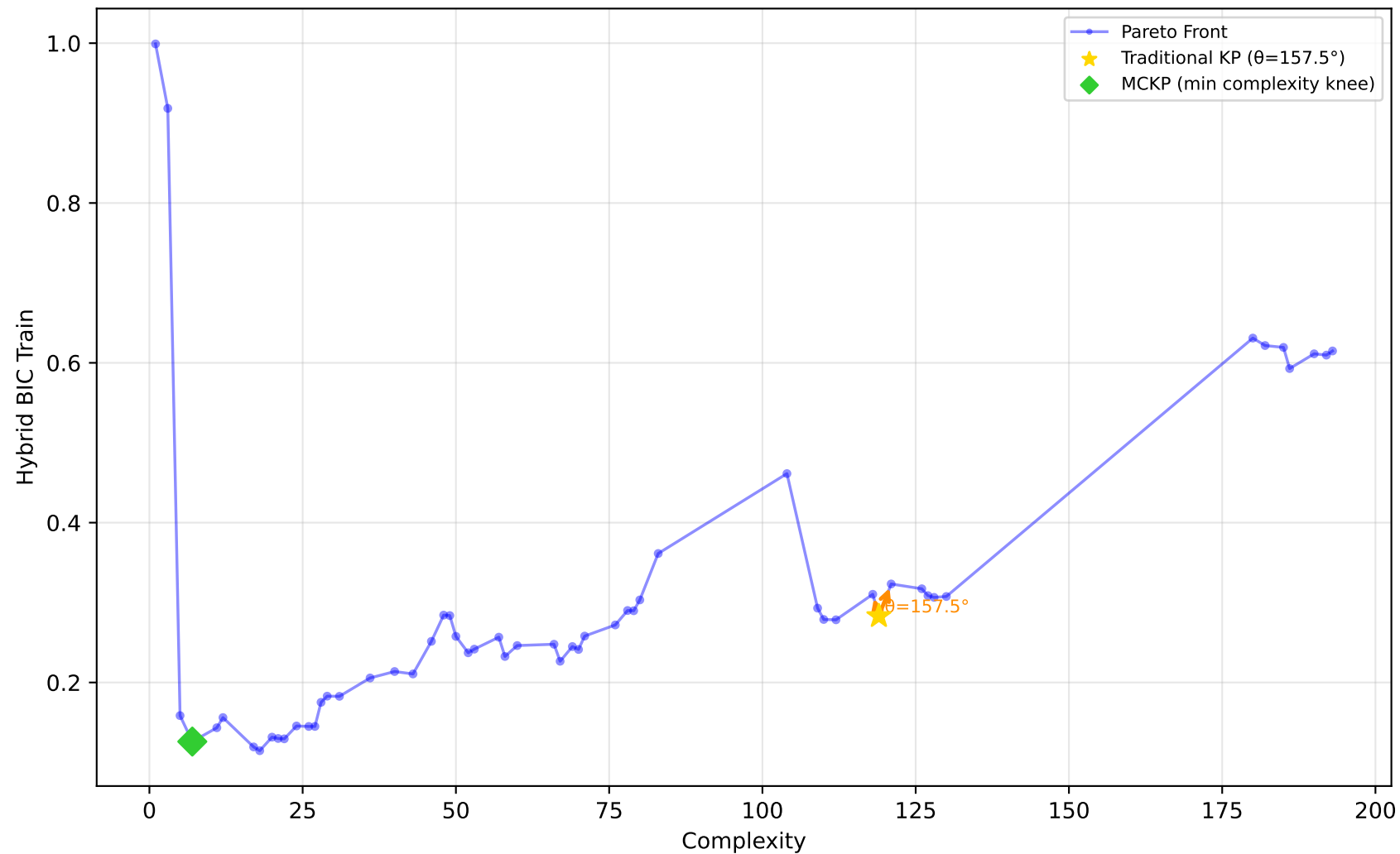
712_chscase_geyser1 - Run 25 - SVP - Hybrid BIC Train \lambda_1=0.00, \lambda_2=1.00, \lambda_3=1.00 | Difficulty: 0.84 | Method: hmr
