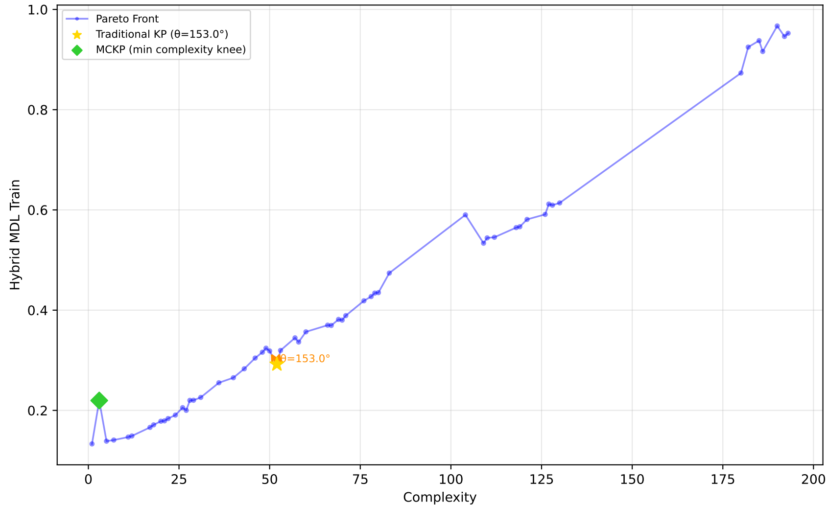
712_chscase_geyser1 - Run 25 - SVP - Hybrid MDL Train \lambda_1=1.00, \lambda_2=1.00, \lambda_3=0.00 | Difficulty: 0.84 | Method: hmr
