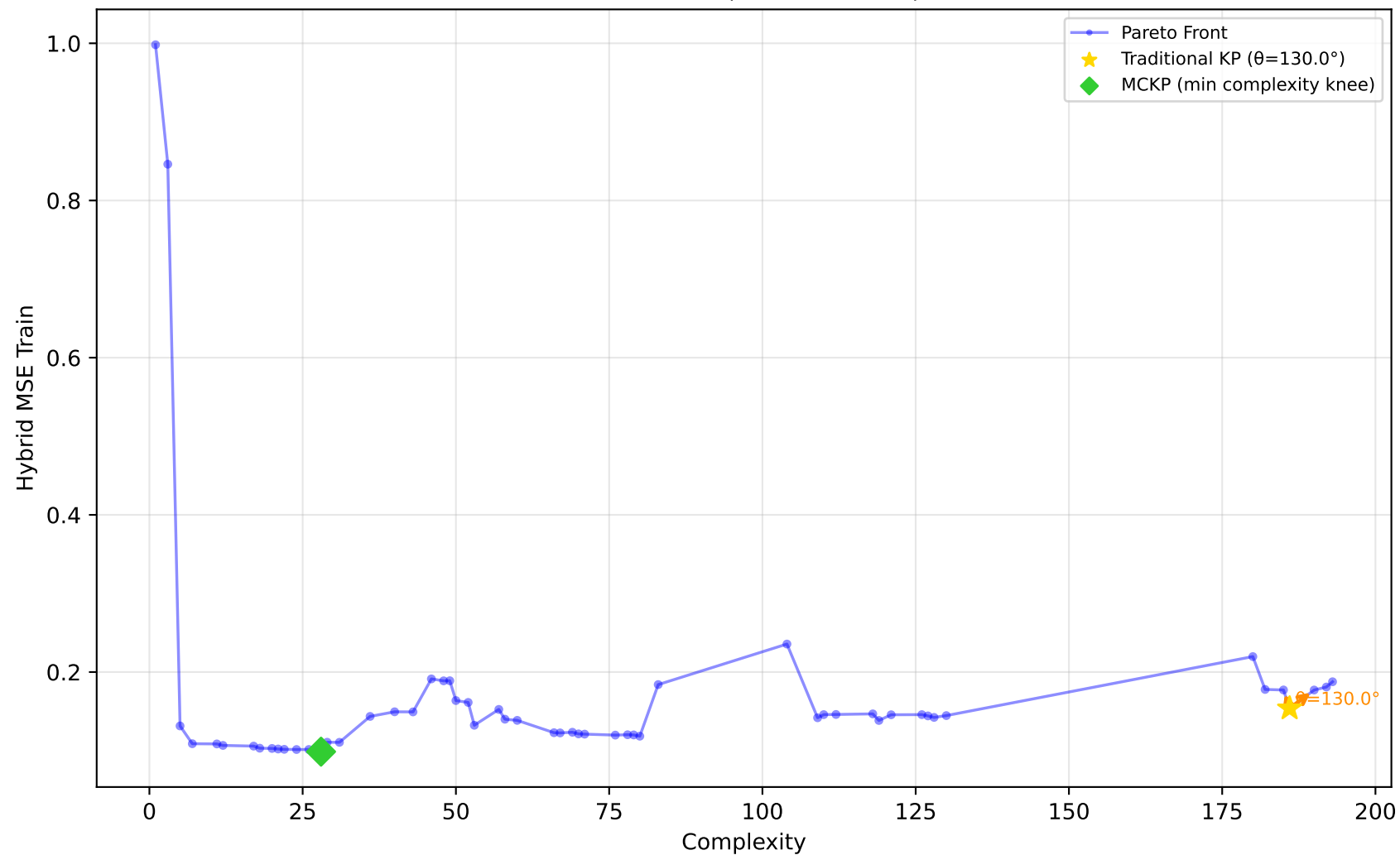
712_chscase_geyser1 - Run 25 - SVP - Hybrid MSE Train \lambda_1=0.00 , \lambda_2=1.00 , \lambda_3=1.00 | Difficulty: 0.84 | Method: hmr
