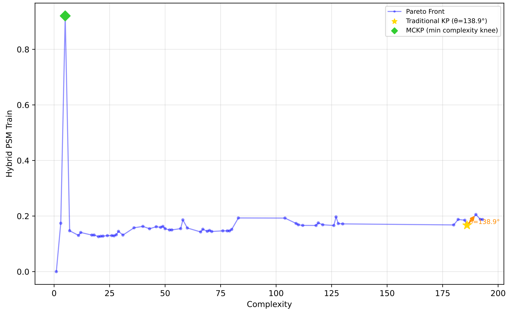
712_chscase_geyser1 - Run 25 - SVP - Hybrid PSM Train \lambda_1=1.00, \lambda_2=1.00, \lambda_3=0.00 | Difficulty: 0.84 | Method: hmr
