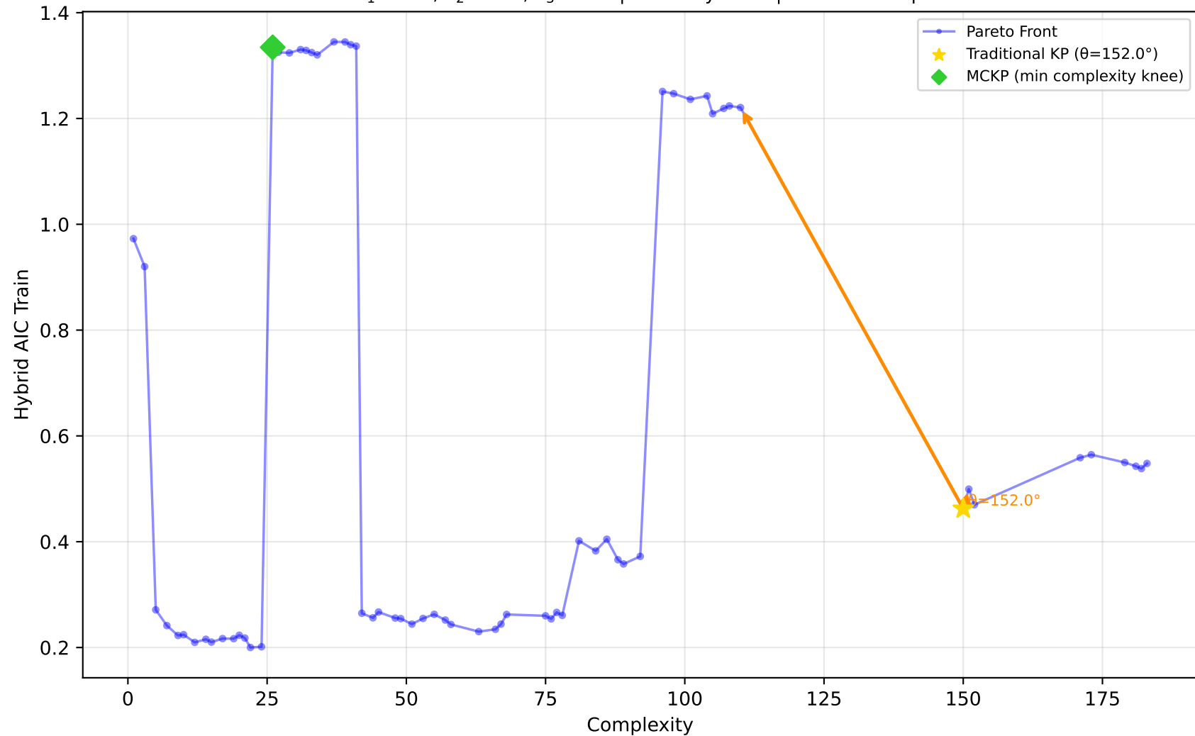
712_chscase_geyser1 - Run 26 - MVP - Hybrid AIC Train \lambda_1=0.20 , \lambda_2=1.00 , \lambda_3=1.00 | Difficulty: 0.59 | Method: mckp
