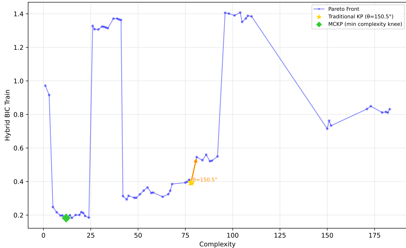
712_chscase_geyser1 - Run 26 - MVP - Hybrid BIC Train \lambda_1=0.20 , \lambda_2=1.00 , \lambda_3=1.00 | Difficulty: 0.59 | Method: mckp
