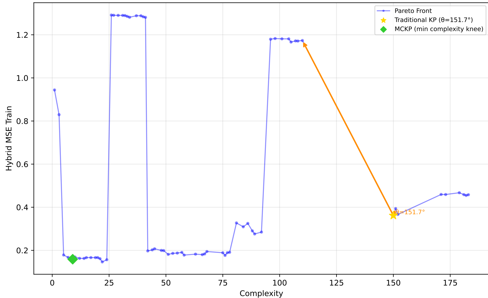
712_chscase_geyser1 - Run 26 - MVP - Hybrid MSE Train \lambda_1=0.20 , \lambda_2=1.00 , \lambda_3=1.00 | Difficulty: 0.59 | Method: mckp
