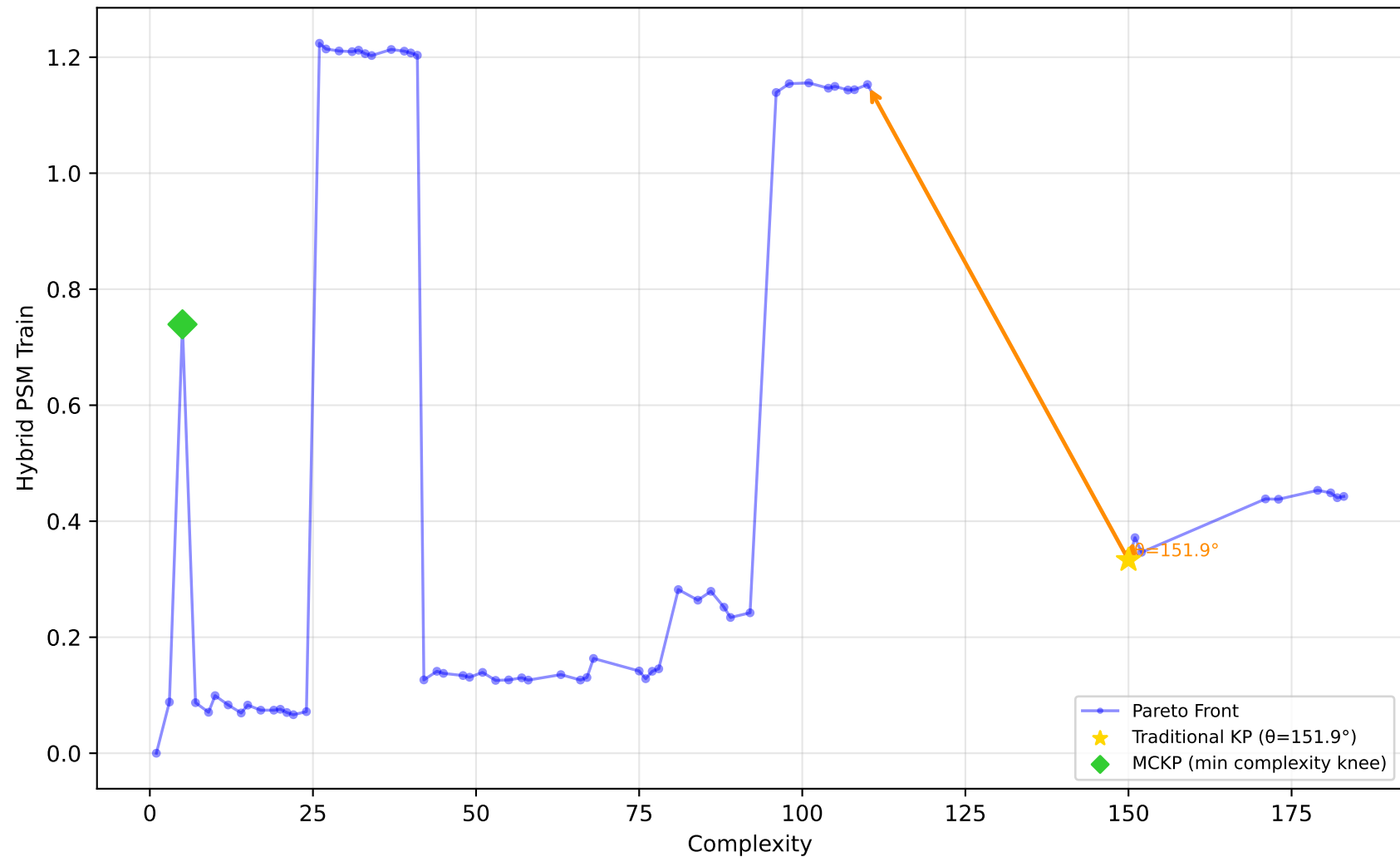
712_chscase_geyser1 - Run 26 - MVP - Hybrid PSM Train \lambda_1=0.20 , \lambda_2=1.00 , \lambda_3=1.00 | Difficulty: 0.59 | Method: mckp
