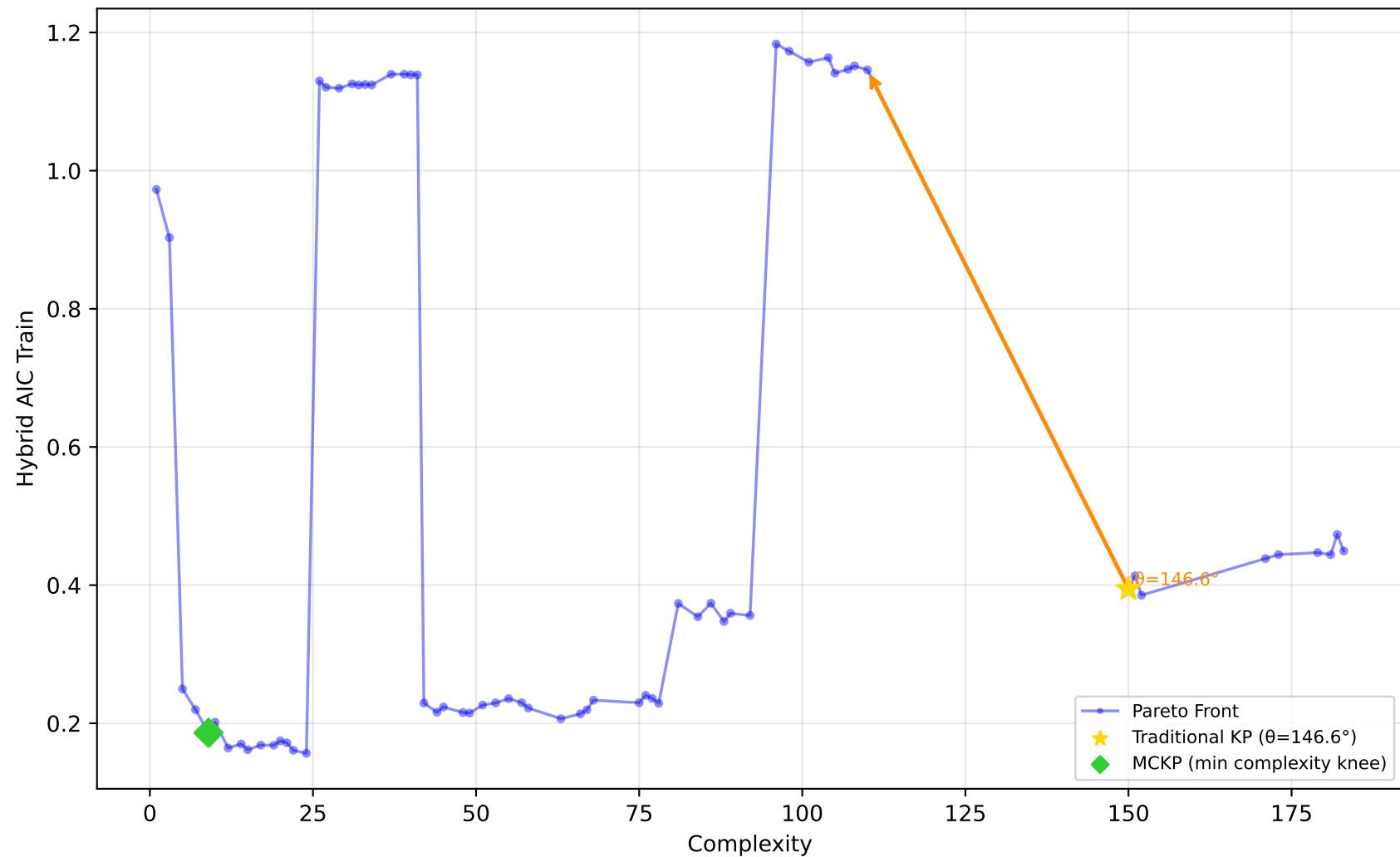
712_chscase_geyser1 - Run 26 - SVP - Hybrid AIC Train \lambda_1=0.00 , \lambda_2=1.00 , \lambda_3=1.00 | Difficulty: 0.59 | Method: mckp
