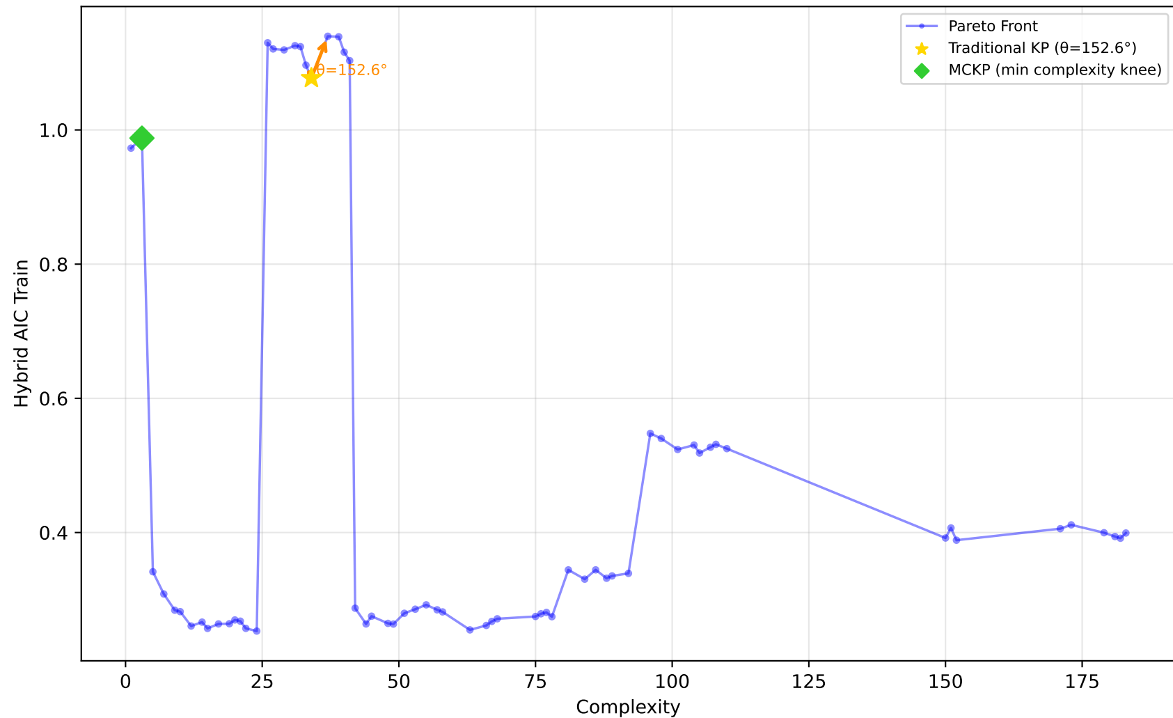
712_chscase_geyser1 - Run 26 - SVP - Hybrid AIC Train \lambda_1=1.00, \lambda_2=1.00, \lambda_3=0.00 | Difficulty: 0.59 | Method: mckp
