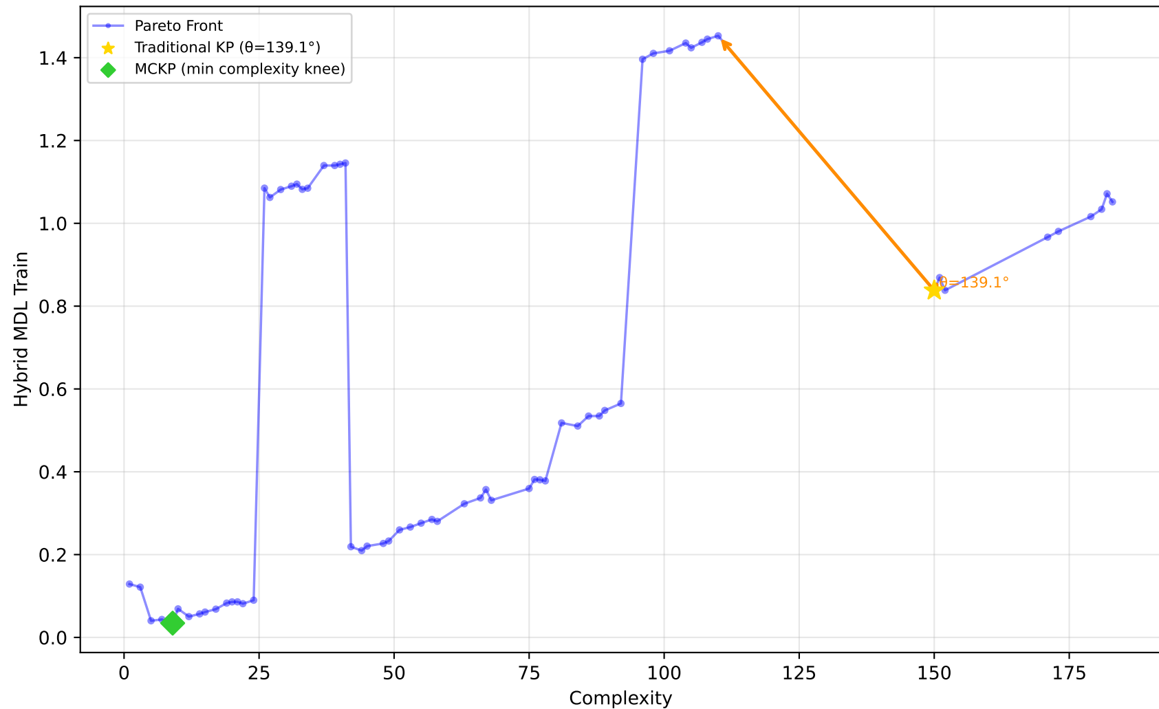
712_chscase_geyser1 - Run 26 - SVP - Hybrid MDL Train \lambda_1=0.00, \lambda_2=1.00, \lambda_3=1.00 | Difficulty: 0.59 | Method: mckp
