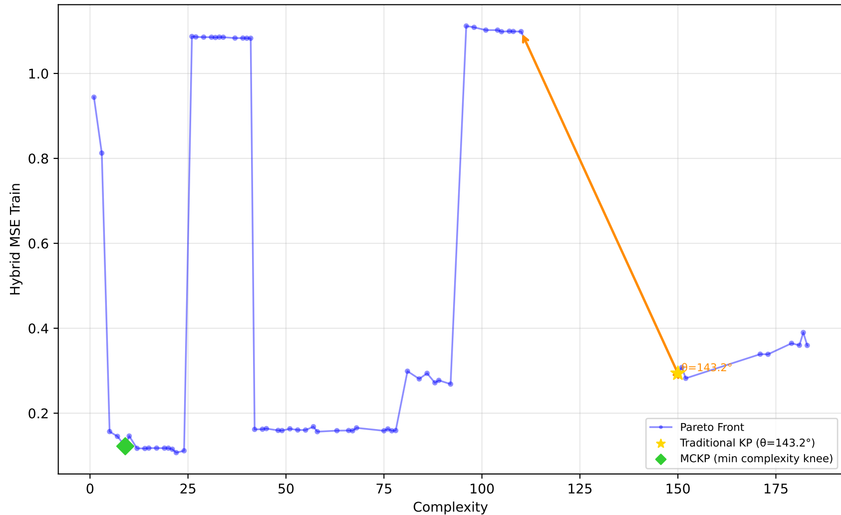
712_chscase_geyser1 - Run 26 - SVP - Hybrid MSE Train \lambda_1=0.00 , \lambda_2=1.00 , \lambda_3=1.00 | Difficulty: 0.59 | Method: mckp
