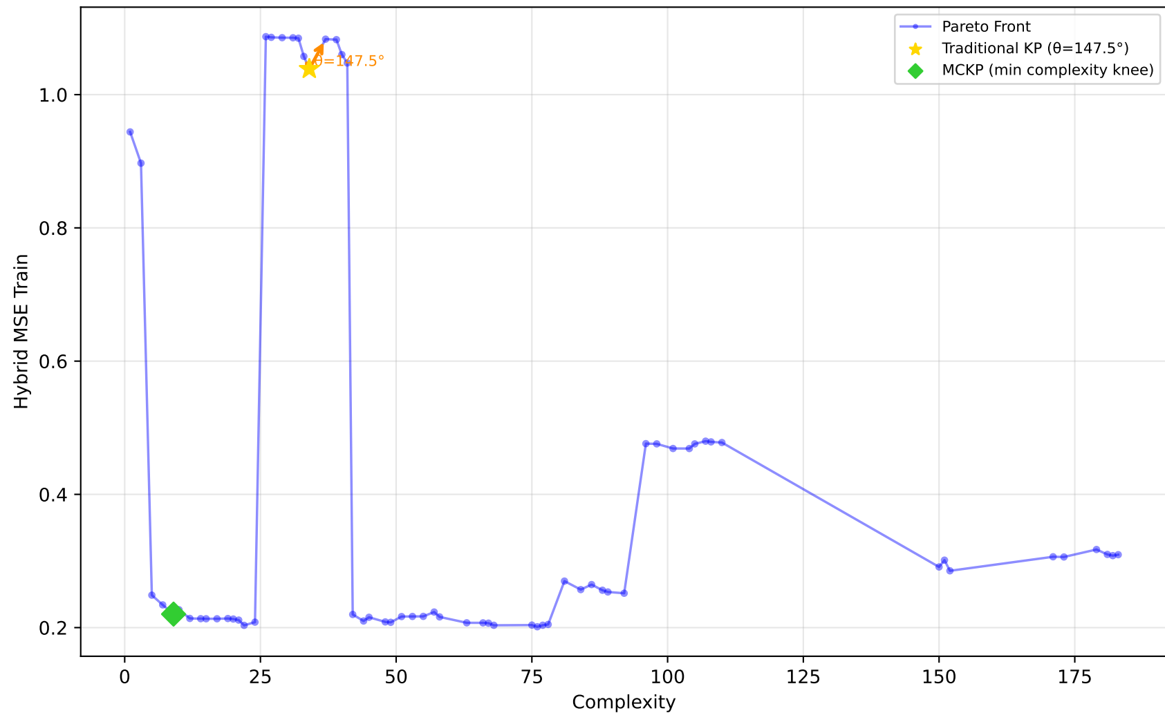
712_chscase_geyser1 - Run 26 - SVP - Hybrid MSE Train \lambda_1=1.00, \lambda_2=1.00, \lambda_3=0.00 | Difficulty: 0.59 | Method: mckp
