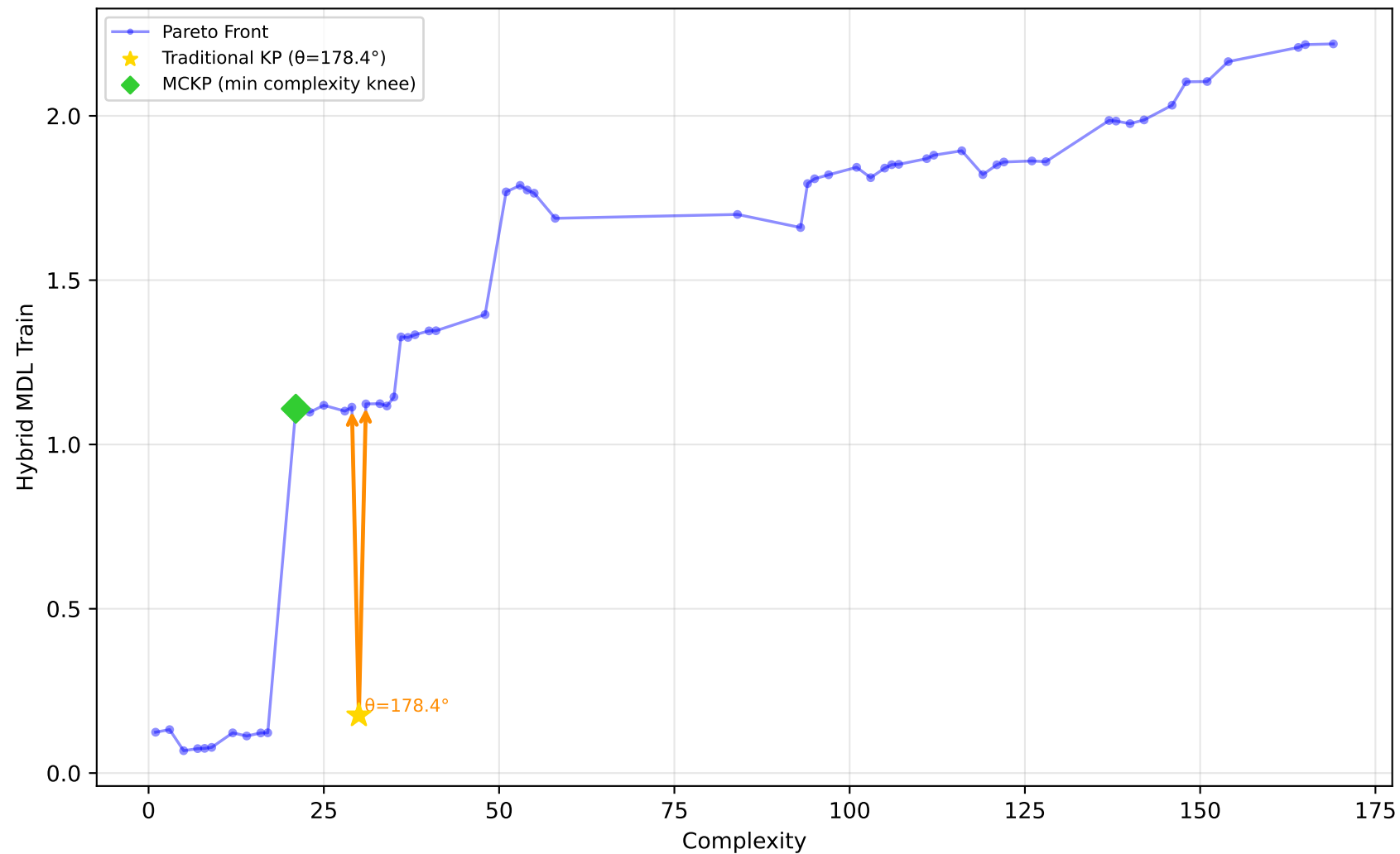
712_chscase_geyser1 - Run 27 - MVP - Hybrid MDL Train \lambda_1=0.20 , \lambda_2=1.00 , \lambda_3=1.00 | Difficulty: 0.34 | Method: mckp
