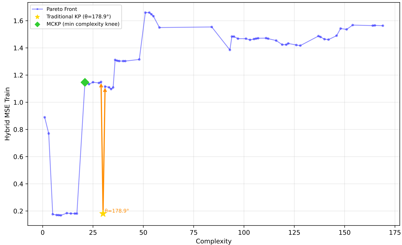
712_chscase_geyser1 - Run 27 - MVP - Hybrid MSE Train \lambda_1=0.20 , \lambda_2=1.00 , \lambda_3=1.00 | Difficulty: 0.34 | Method: mckp
