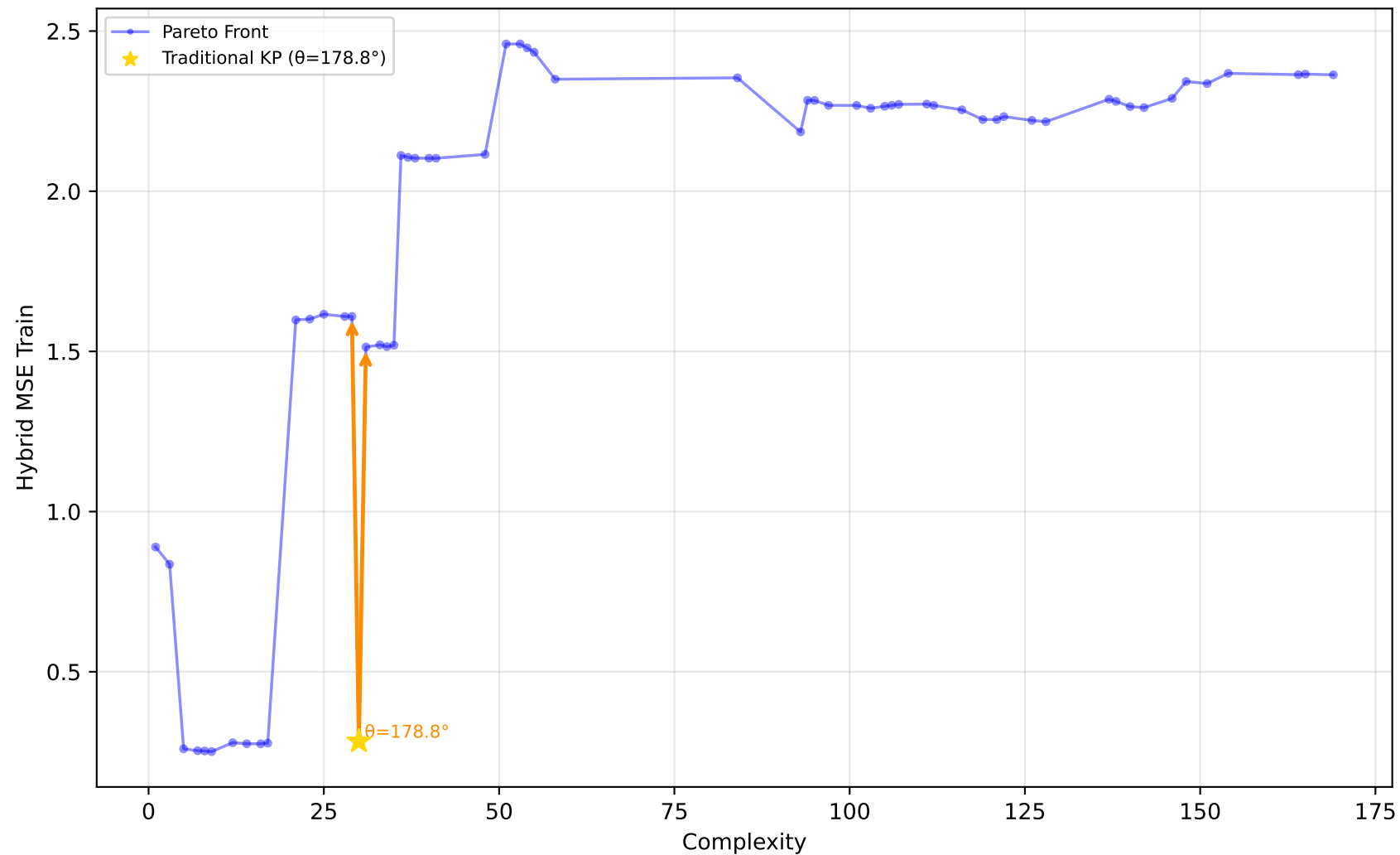
712_chscase_geyser1 - Run 27 - MVP - Hybrid MSE Train \lambda_1=1.00, \lambda_2=1.00, \lambda_3=1.00 | Difficulty: 0.34 | Method: mckp
