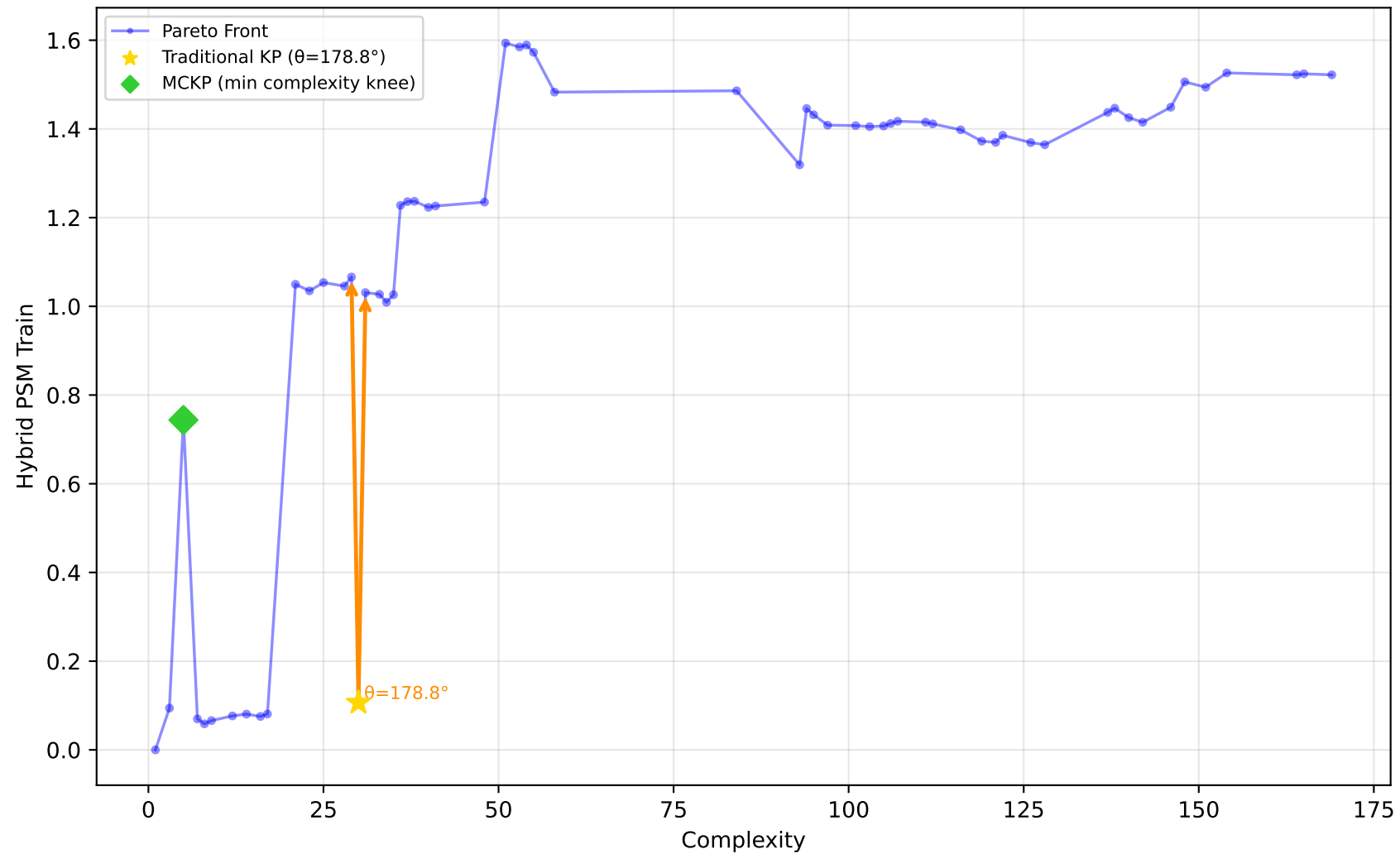
712_chscase_geyser1 - Run 27 - MVP - Hybrid PSM Train \lambda_1=0.20 , \lambda_2=1.00 , \lambda_3=1.00 | Difficulty: 0.34 | Method: mckp
