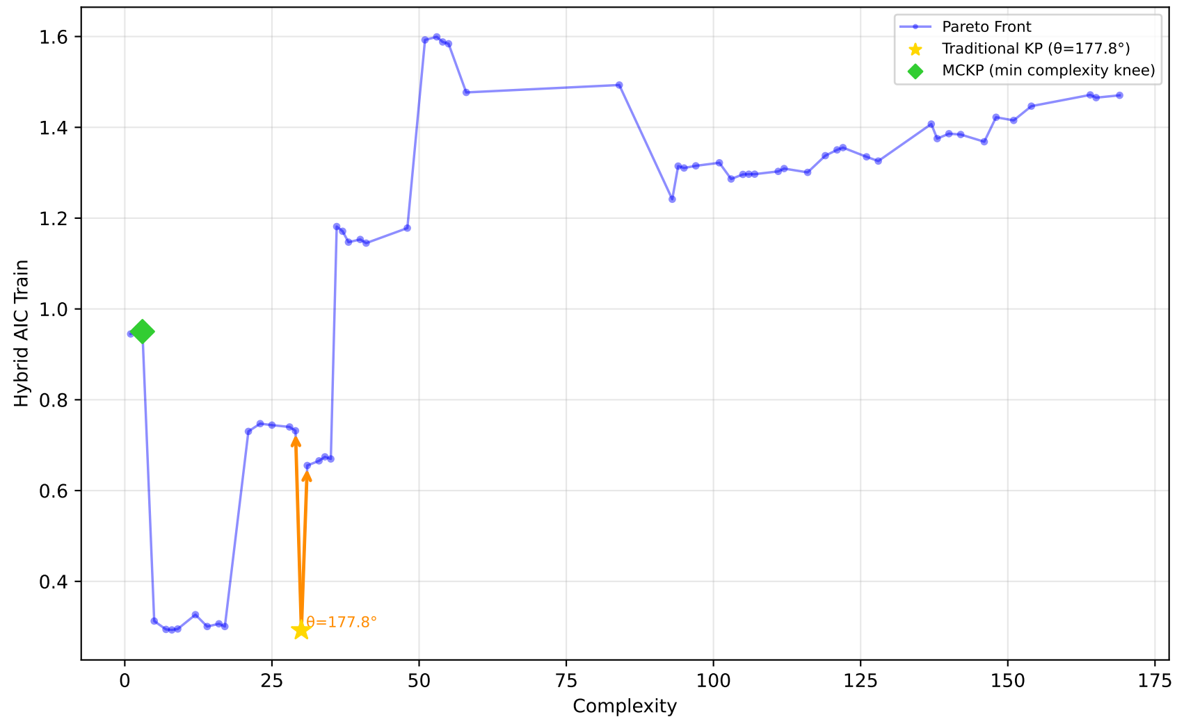
712_chscase_geyser1 - Run 27 - SVP - Hybrid AIC Train \lambda_1=1.00 , \lambda_2=1.00 , \lambda_3=0.00 | Difficulty: 0.34 | Method: mckp
