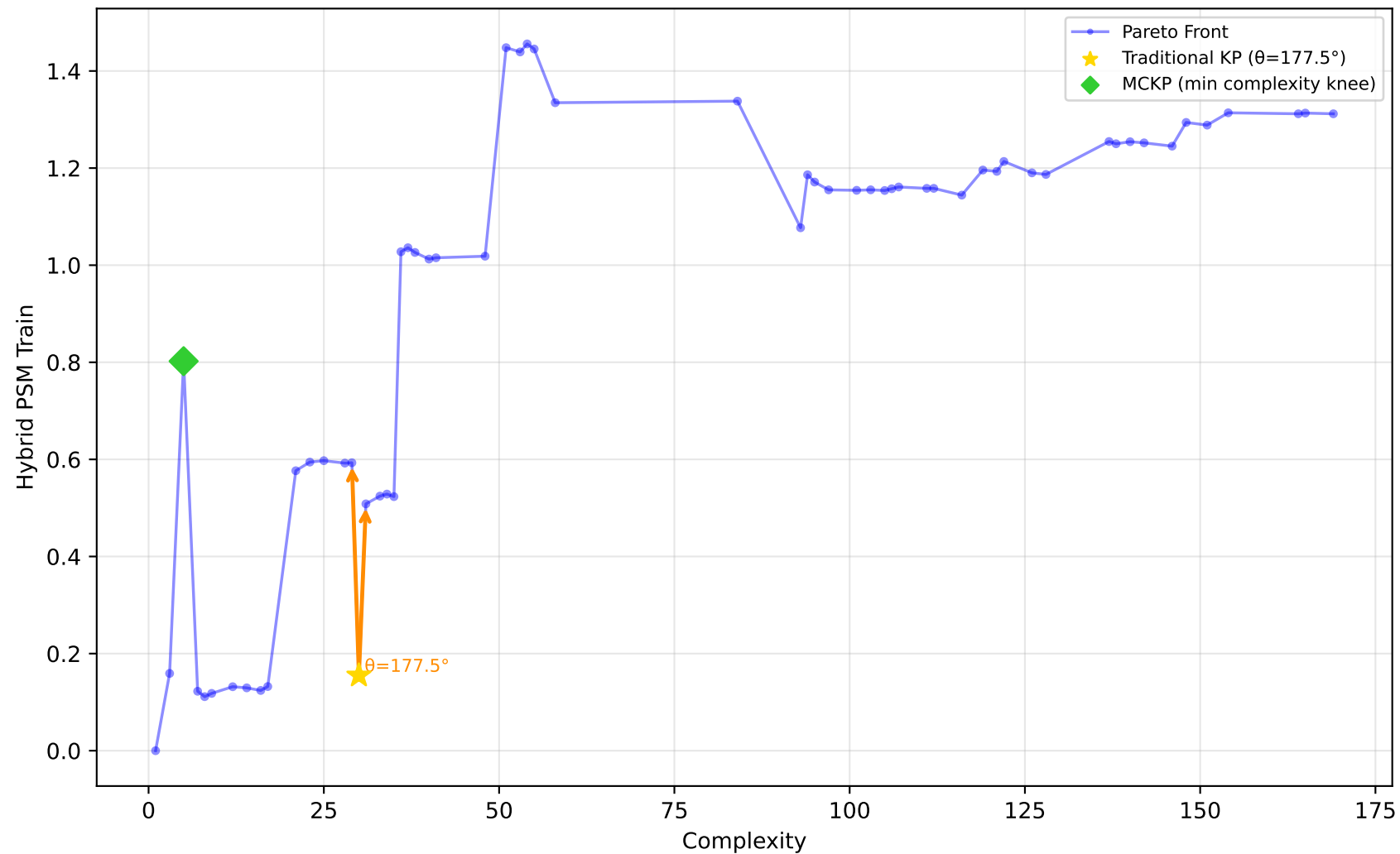
712_chscase_geyser1 - Run 27 - SVP - Hybrid PSM Train \lambda_1=1.00 , \lambda_2=1.00 , \lambda_3=0.00 | Difficulty: 0.34 | Method: mckp
