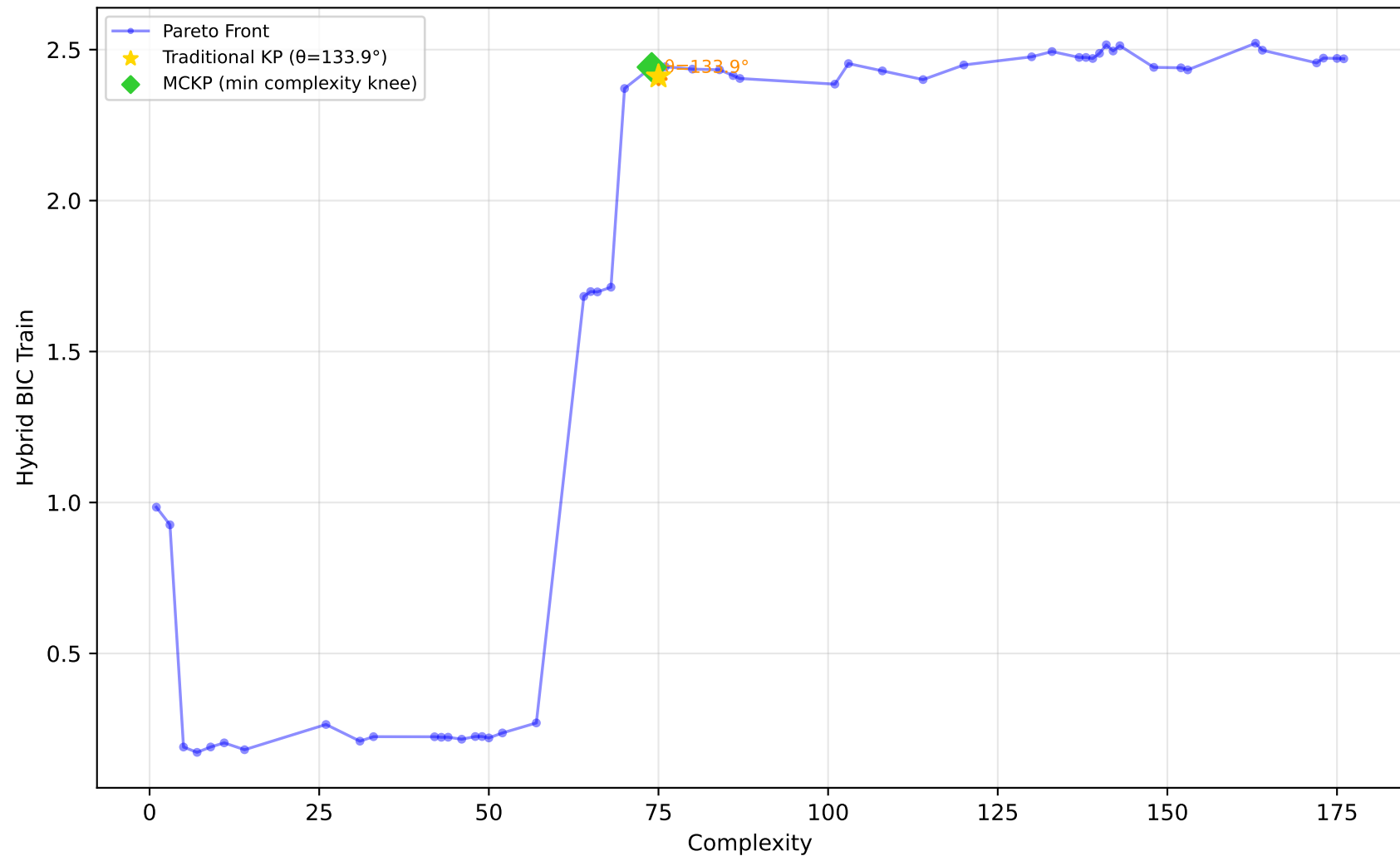
712_chscase_geyser1 - Run 28 - MVP - Hybrid BIC Train \lambda_1=0.20, \lambda_2=1.00, \lambda_3=1.00 | Difficulty: 0.39 | Method: mckp
