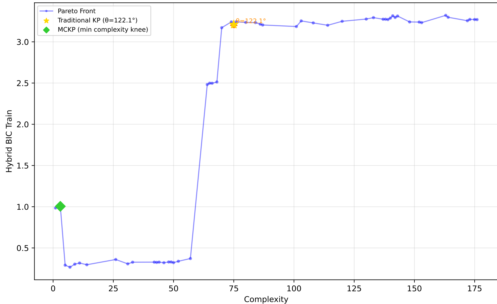
712_chscase_geyser1 - Run 28 - MVP - Hybrid BIC Train \lambda_1=1.00, \lambda_2=1.00, \lambda_3=1.00 | Difficulty: 0.39 | Method: mckp
