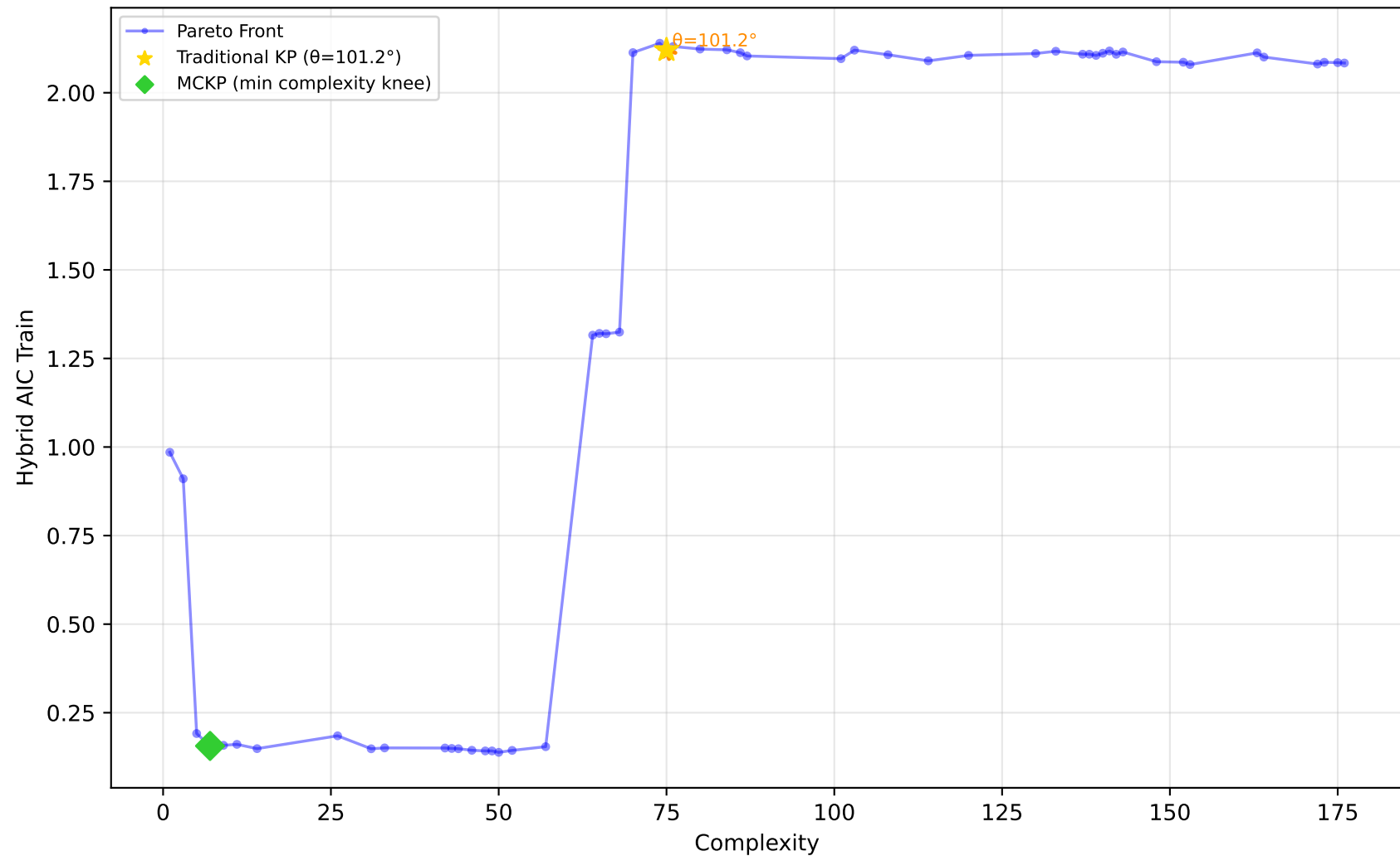
712_chscase_geyser1 - Run 28 - SVP - Hybrid AIC Train \lambda_1=0.00, \lambda_2=1.00, \lambda_3=1.00 | Difficulty: 0.39 | Method: mckp
