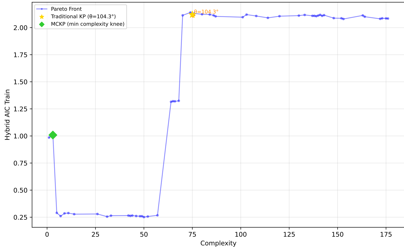
712_chscase_geyser1 - Run 28 - SVP - Hybrid AIC Train \lambda_1=1.00, \lambda_2=1.00, \lambda_3=0.00 | Difficulty: 0.39 | Method: mckp
