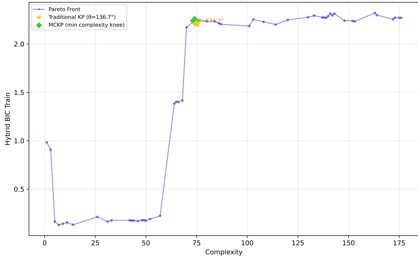
712_chscase_geyser1 - Run 28 - SVP - Hybrid BIC Train \lambda_1=0.00, \lambda_2=1.00, \lambda_3=1.00 | Difficulty: 0.39 | Method: mckp
