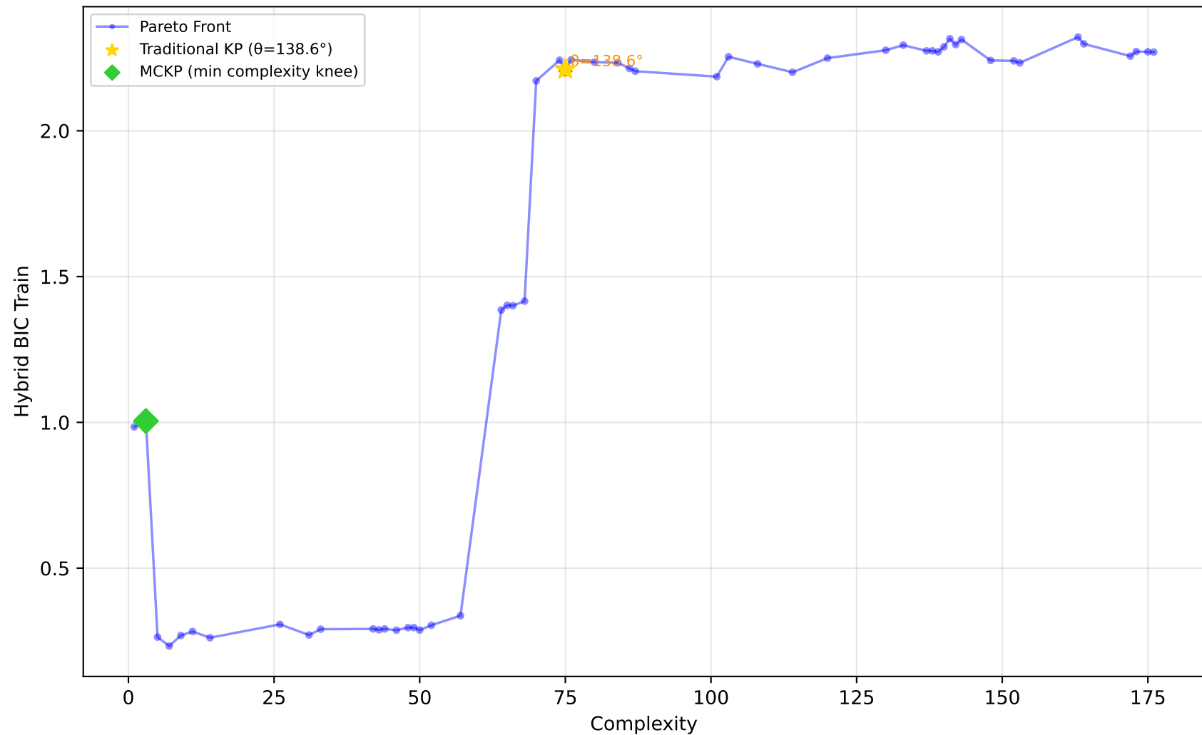
712_chscase_geyser1 - Run 28 - SVP - Hybrid BIC Train \lambda_1=1.00, \lambda_2=1.00, \lambda_3=0.00 | Difficulty: 0.39 | Method: mckp
