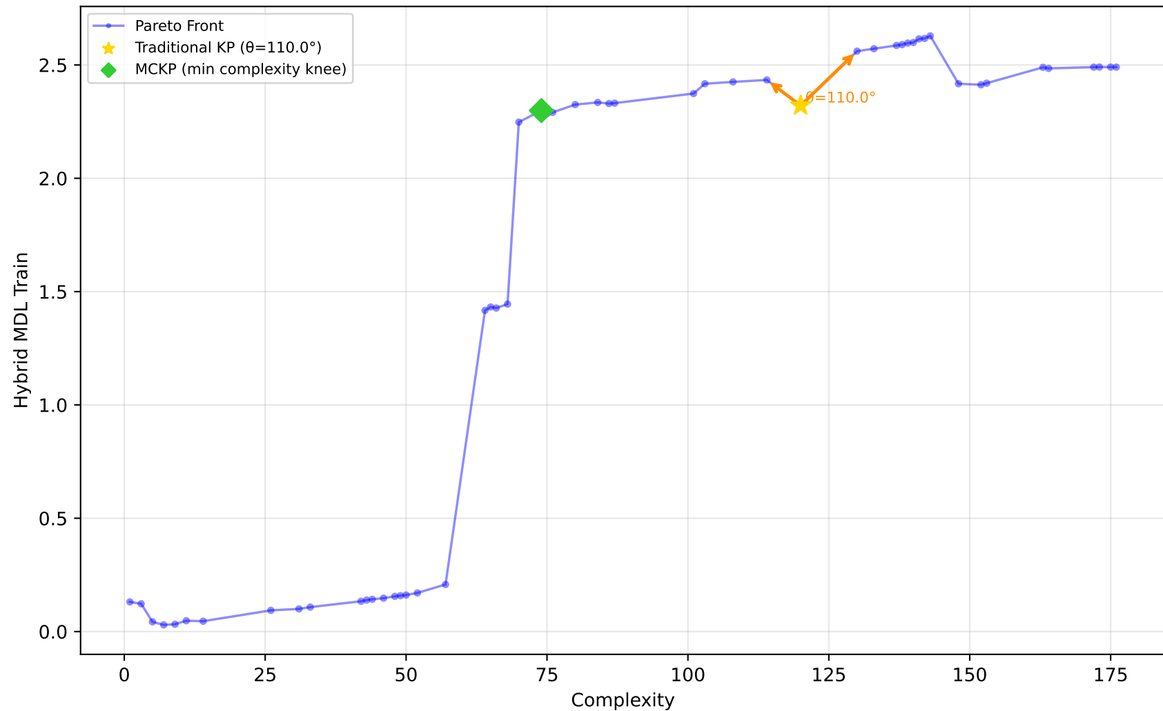
712_chscase_geyser1 - Run 28 - SVP - Hybrid MDL Train \lambda_1=0.00 , \lambda_2=1.00 , \lambda_3=1.00 | Difficulty: 0.39 | Method: mckp
