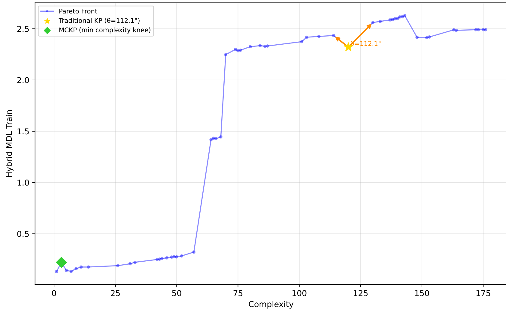
712_chscase_geyser1 - Run 28 - SVP - Hybrid MDL Train \lambda_1=1.00, \lambda_2=1.00, \lambda_3=0.00 | Difficulty: 0.39 | Method: mckp
