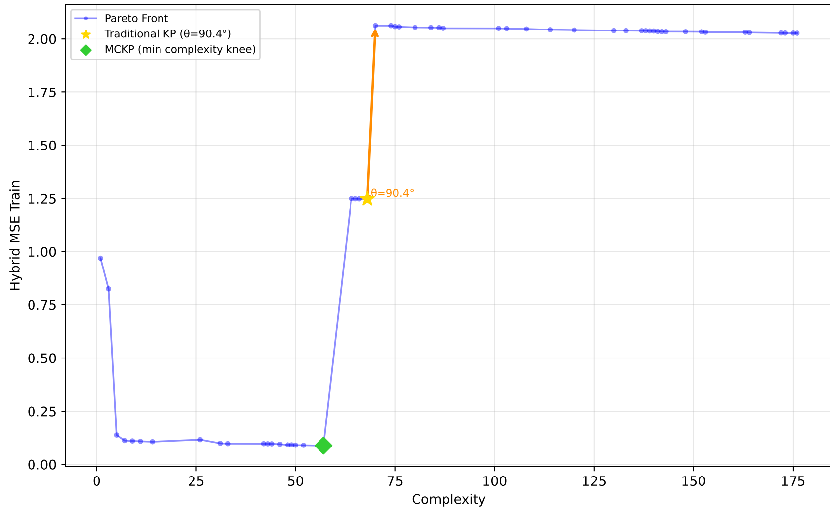
712_chscase_geyser1 - Run 28 - SVP - Hybrid MSE Train \lambda_1=0.00, \lambda_2=1.00, \lambda_3=1.00 | Difficulty: 0.39 | Method: mckp
