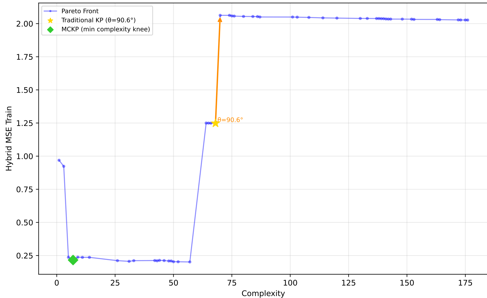
712_chscase_geyser1 - Run 28 - SVP - Hybrid MSE Train \lambda_1=1.00, \lambda_2=1.00, \lambda_3=0.00 | Difficulty: 0.39 | Method: mckp
