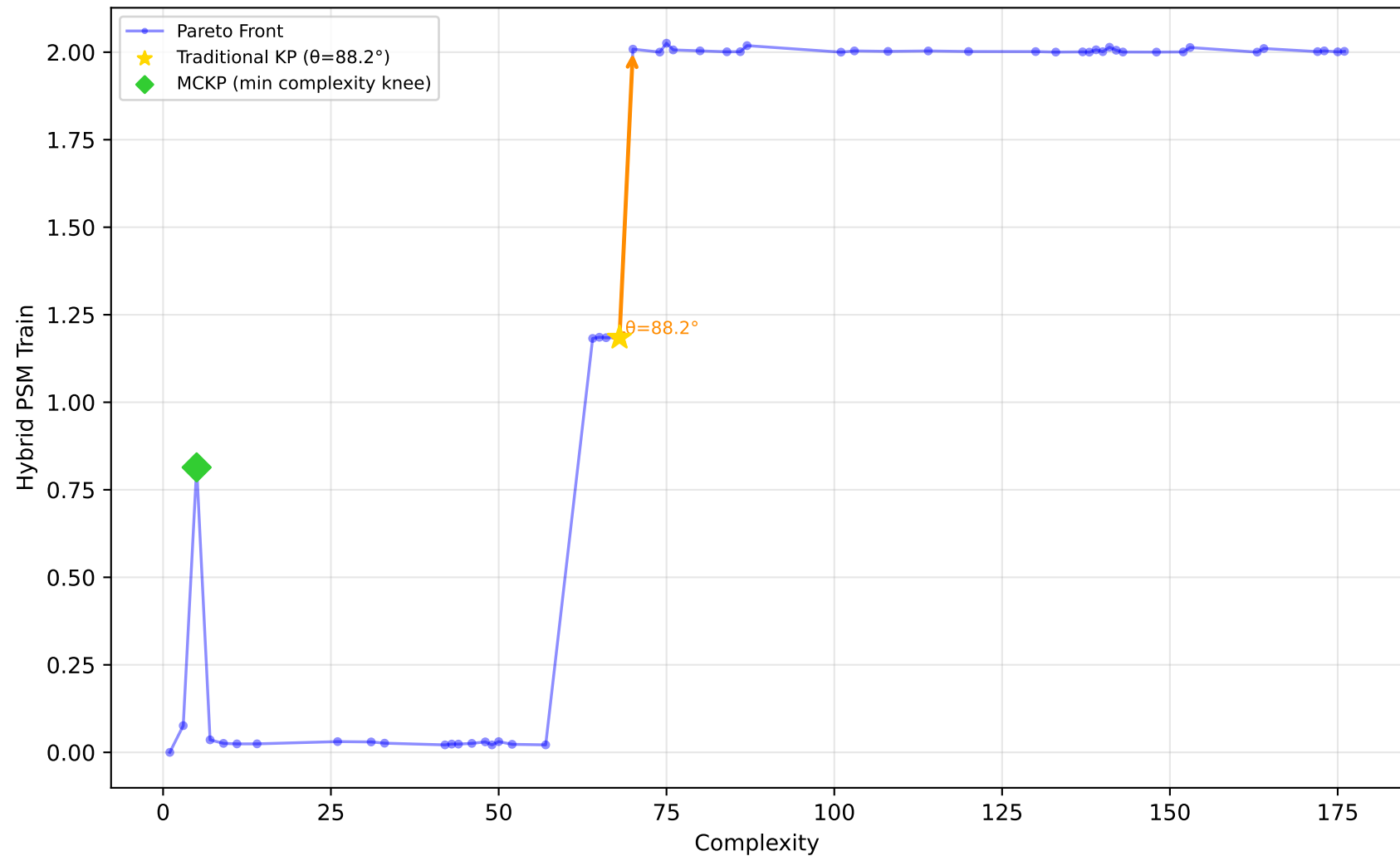
712_chscase_geyser1 - Run 28 - SVP - Hybrid PSM Train \lambda_1=0.00, \lambda_2=1.00, \lambda_3=1.00 | Difficulty: 0.39 | Method: mckp
