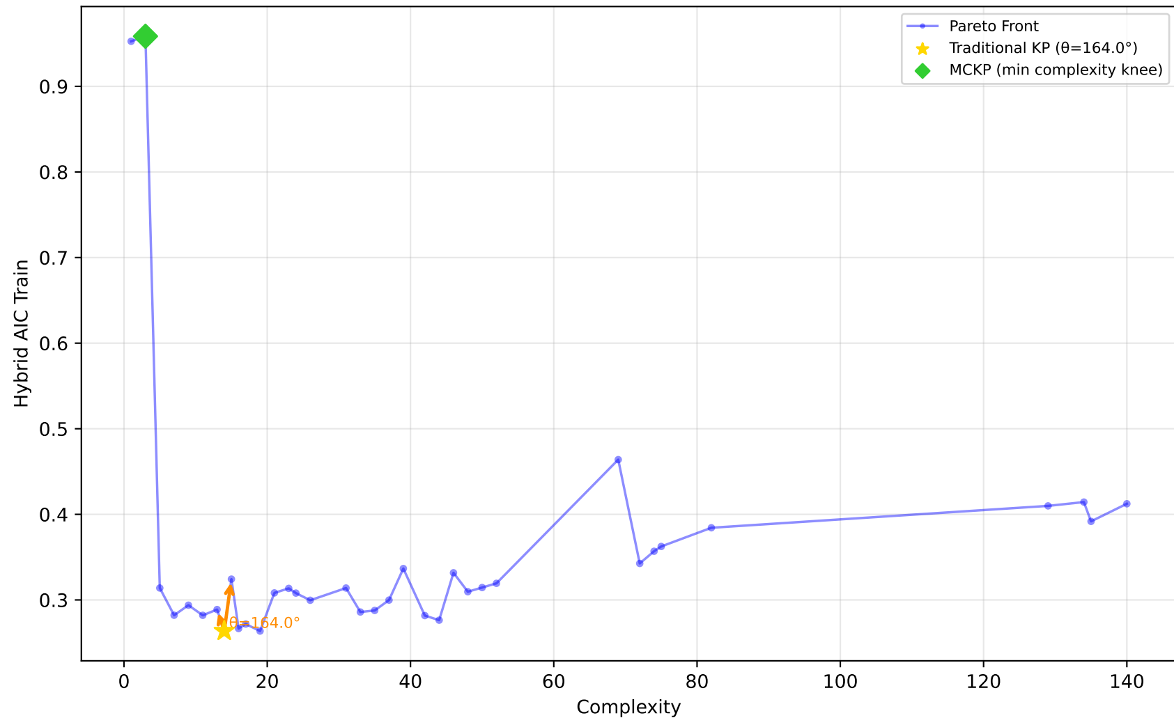
712_chscase_geyser1 - Run 29 - MVP - Hybrid AIC Train \lambda_1=1.00, \lambda_2=1.00, \lambda_3=1.00 | Difficulty: 0.54 | Method: mckp
