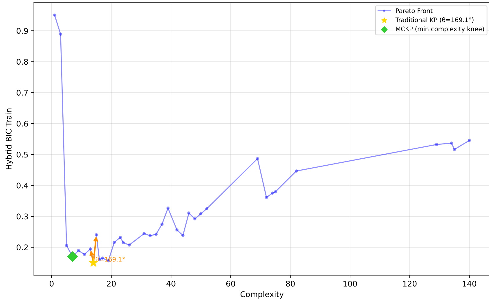
712_chscase_geyser1 - Run 29 - MVP - Hybrid BIC Train \lambda_1=0.20 , \lambda_2=1.00 , \lambda_3=1.00 | Difficulty: 0.54 | Method: mckp
