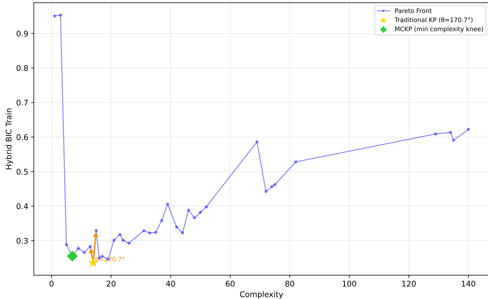
712_chscase_geyser1 - Run 29 - MVP - Hybrid BIC Train \lambda_1=1.00, \lambda_2=1.00, \lambda_3=1.00 | Difficulty: 0.54 | Method: mckp
