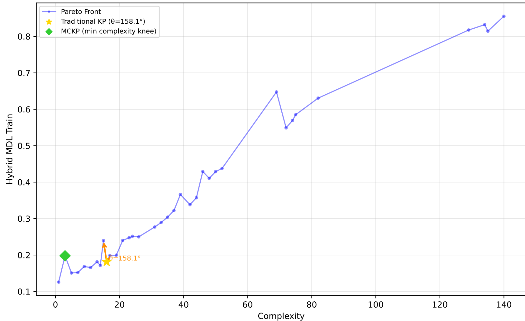
712_chscase_geyser1 - Run 29 - MVP - Hybrid MDL Train \lambda_1=1.00, \lambda_2=1.00, \lambda_3=1.00 | Difficulty: 0.54 | Method: mckp
