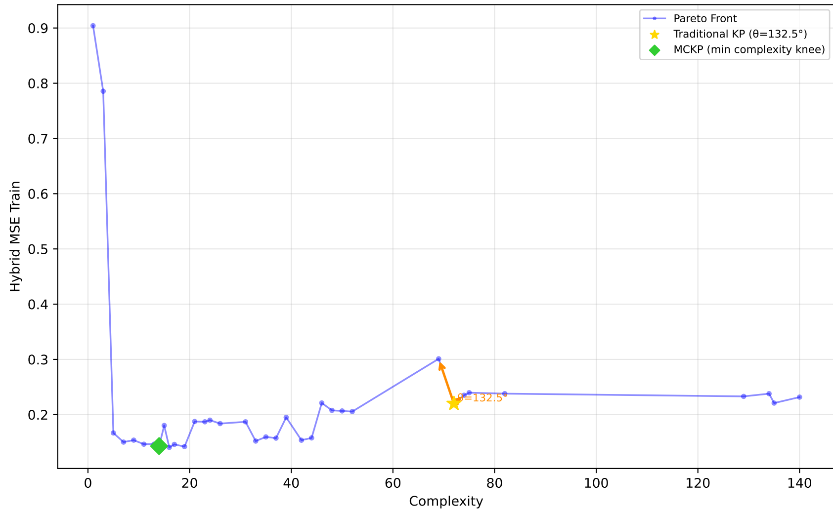
712_chscase_geyser1 - Run 29 - MVP - Hybrid MSE Train \lambda_1=0.20 , \lambda_2=1.00 , \lambda_3=1.00 | Difficulty: 0.54 | Method: mckp
