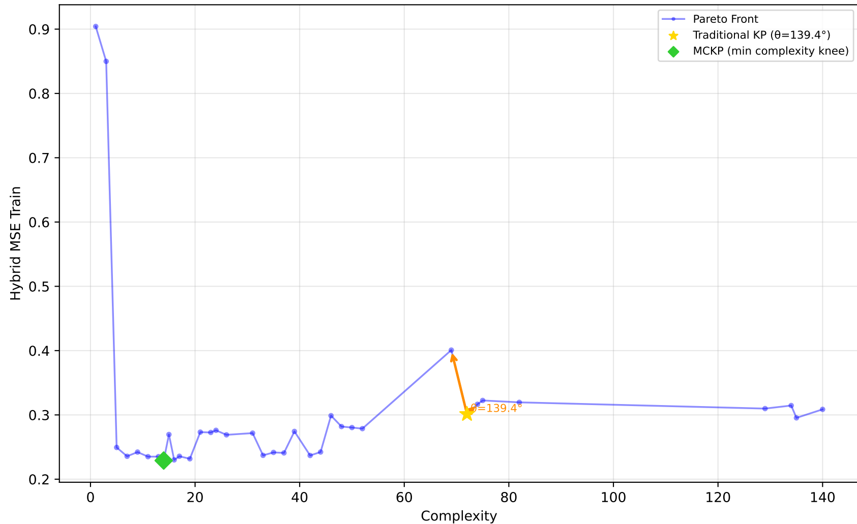
712_chscase_geyser1 - Run 29 - MVP - Hybrid MSE Train \lambda_1=1.00, \lambda_2=1.00, \lambda_3=1.00 | Difficulty: 0.54 | Method: mckp
