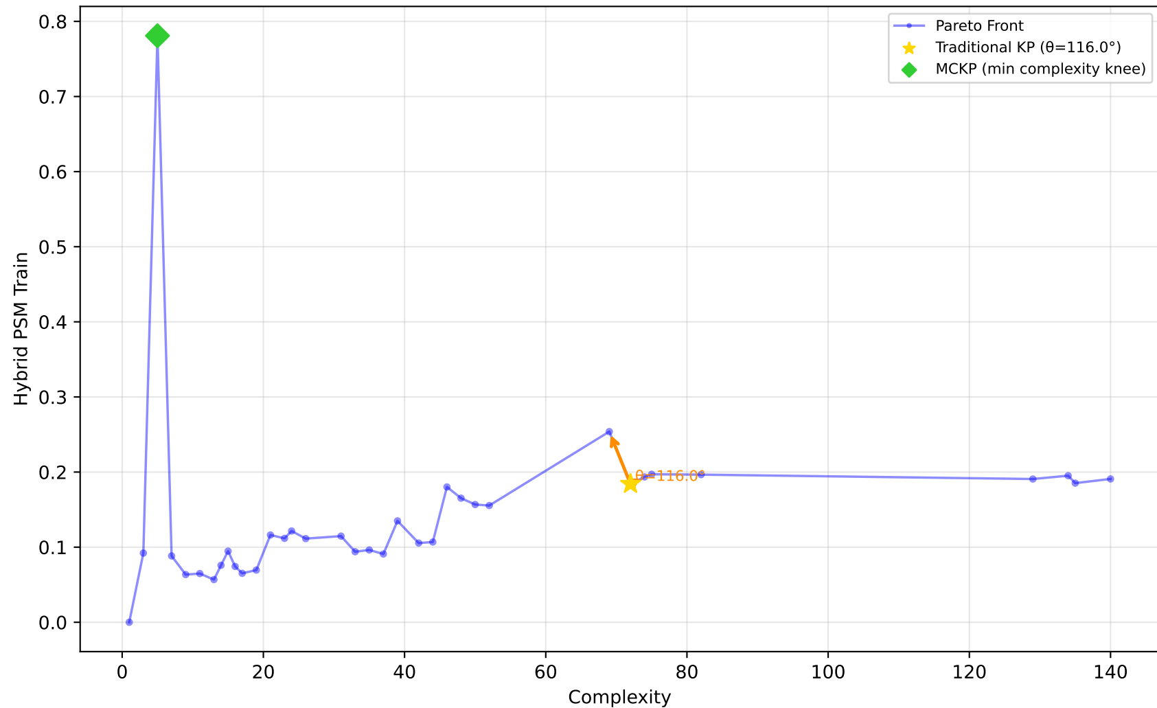
712_chscase_geyser1 - Run 29 - MVP - Hybrid PSM Train \lambda_1=0.20, \lambda_2=1.00, \lambda_3=1.00 | Difficulty: 0.54 | Method: mckp
