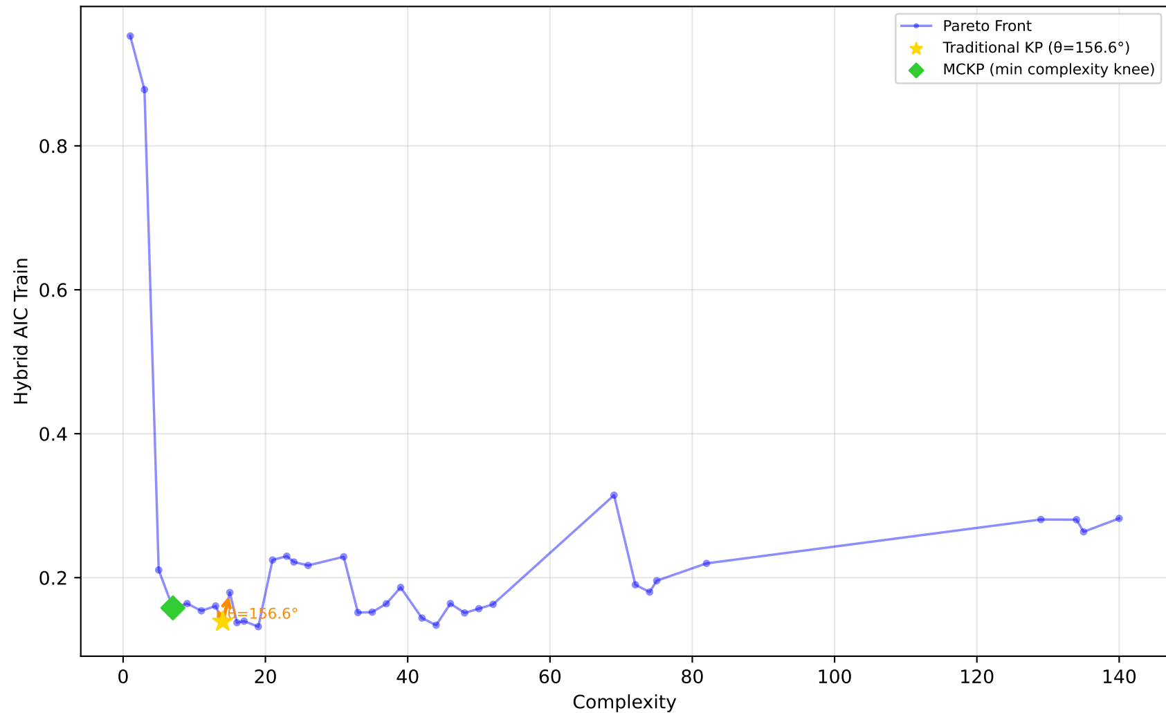
712_chscase_geyser1 - Run 29 - SVP - Hybrid AIC Train \lambda_1=0.00 , \lambda_2=1.00 , \lambda_3=1.00 | Difficulty: 0.54 | Method: mckp
