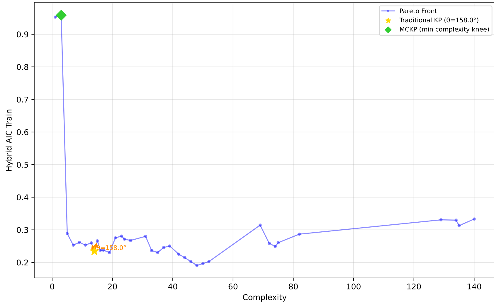
712_chscase_geyser1 - Run 29 - SVP - Hybrid AIC Train \lambda_1=1.00 , \lambda_2=1.00 , \lambda_3=0.00 | Difficulty: 0.54 | Method: mckp
