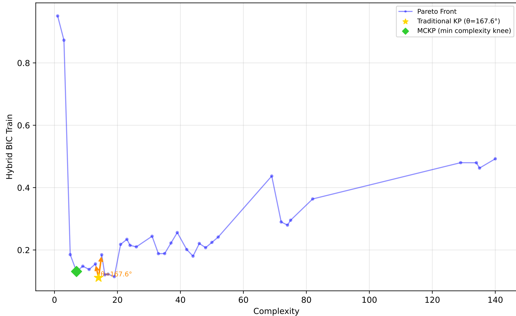
712_chscase_geyser1 - Run 29 - SVP - Hybrid BIC Train \lambda_1=0.00, \lambda_2=1.00, \lambda_3=1.00 | Difficulty: 0.54 | Method: mckp
