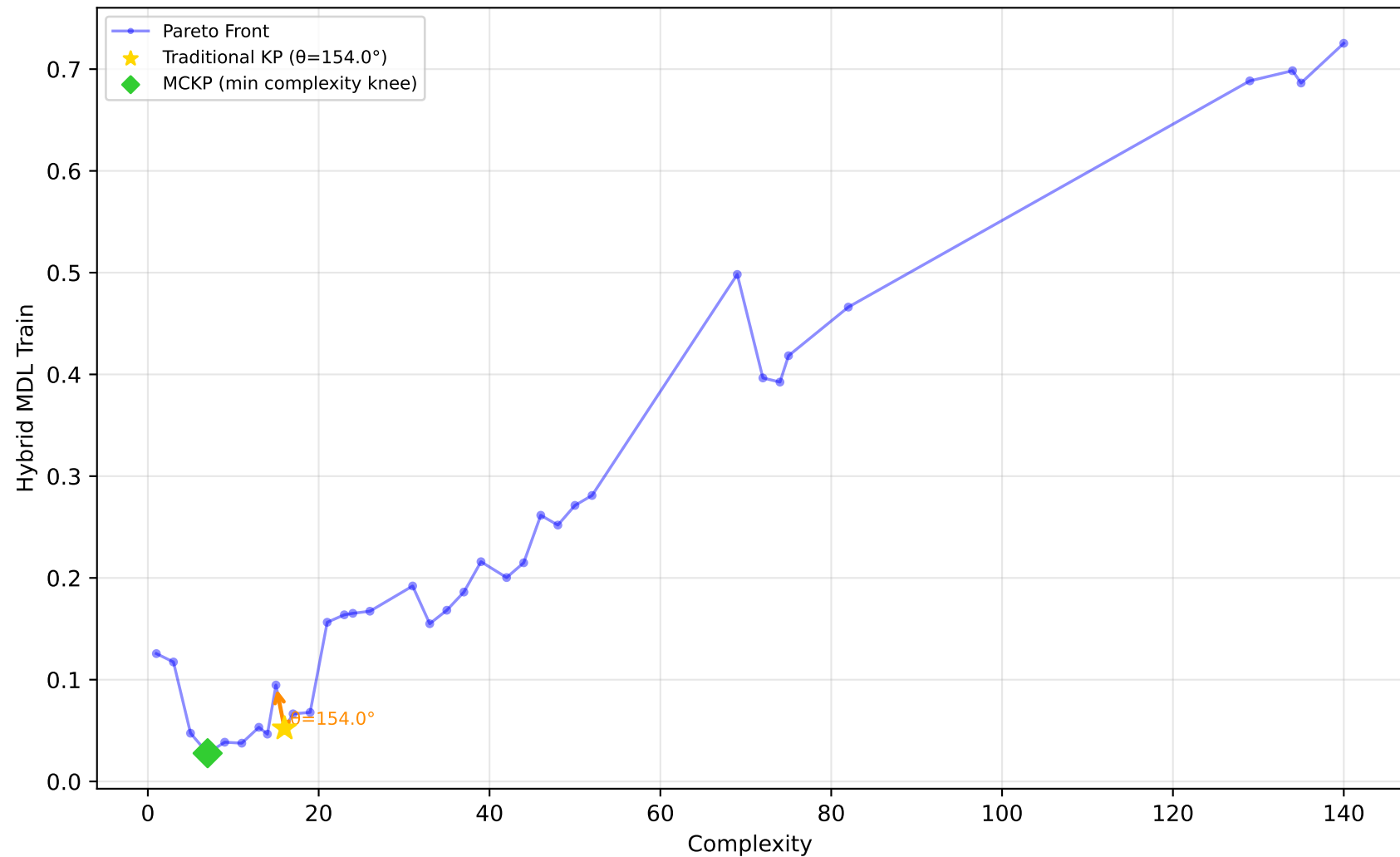
712_chscase_geyser1 - Run 29 - SVP - Hybrid MDL Train \lambda_1=0.00 , \lambda_2=1.00 , \lambda_3=1.00 | Difficulty: 0.54 | Method: mckp
