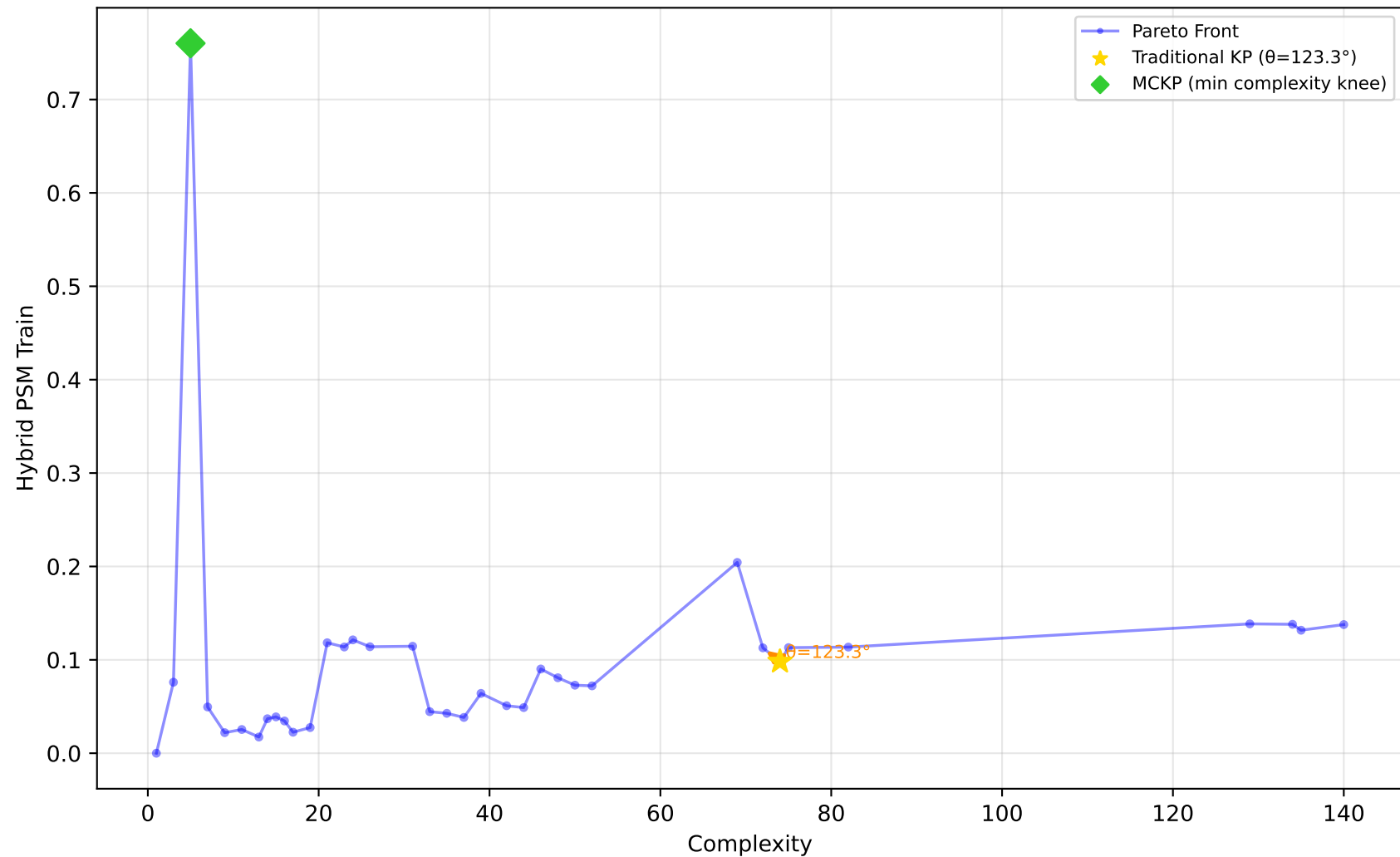
712_chscase_geyser1 - Run 29 - SVP - Hybrid PSM Train \lambda_1=0.00, \lambda_2=1.00, \lambda_3=1.00 | Difficulty: 0.54 | Method: mckp
