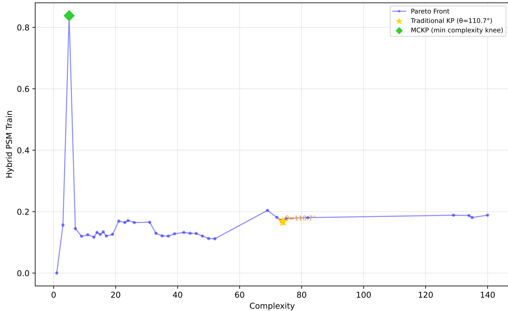
712_chscase_geyser1 - Run 29 - SVP - Hybrid PSM Train \lambda_1=1.00, \lambda_2=1.00, \lambda_3=0.00 | Difficulty: 0.54 | Method: mckp
