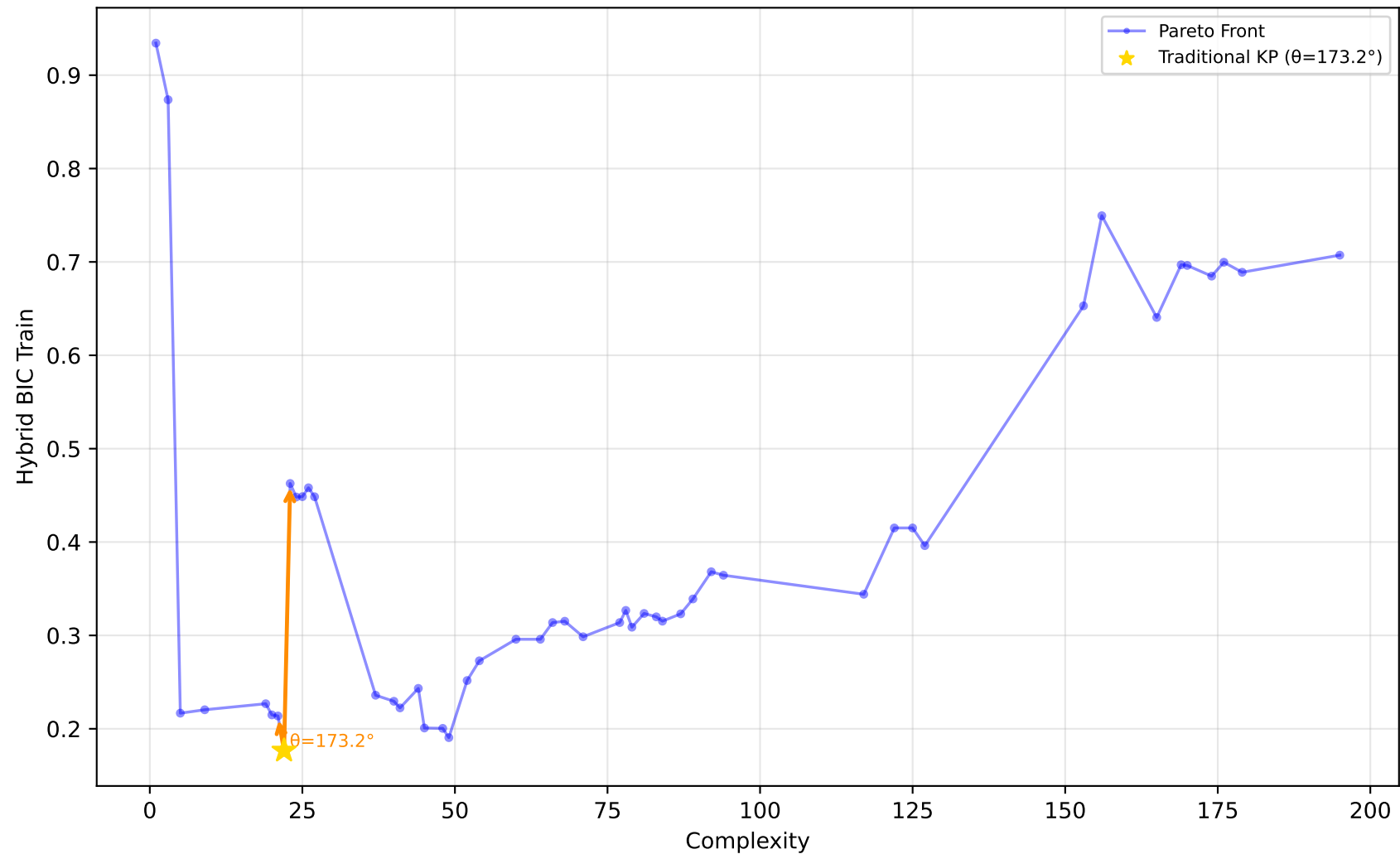
712_chscase_geyser1 - Run 2 - MVP - Hybrid BIC Train \lambda_1=0.20 , \lambda_2=1.00 , \lambda_3=1.00 | Difficulty: 1.00 | Method: hmr
