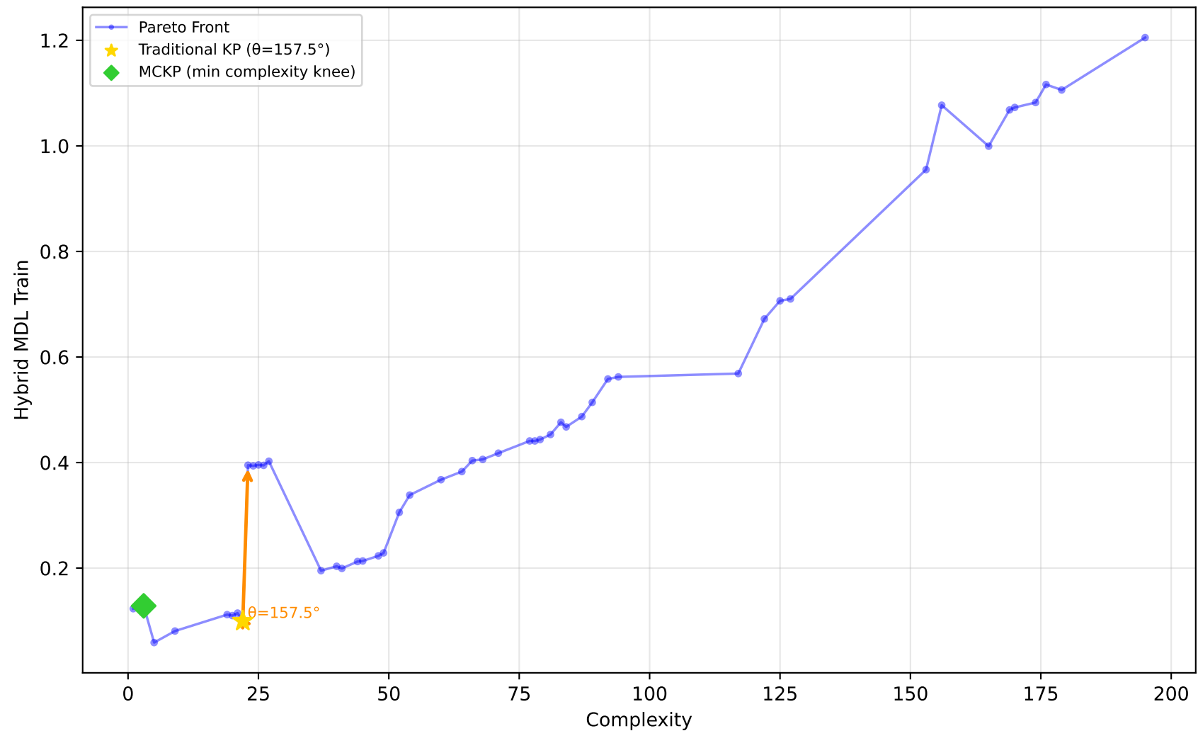
712_chscase_geyser1 - Run 2 - MVP - Hybrid MDL Train \lambda_1=0.20, \lambda_2=1.00, \lambda_3=1.00 | Difficulty: 1.00 | Method: hmr
