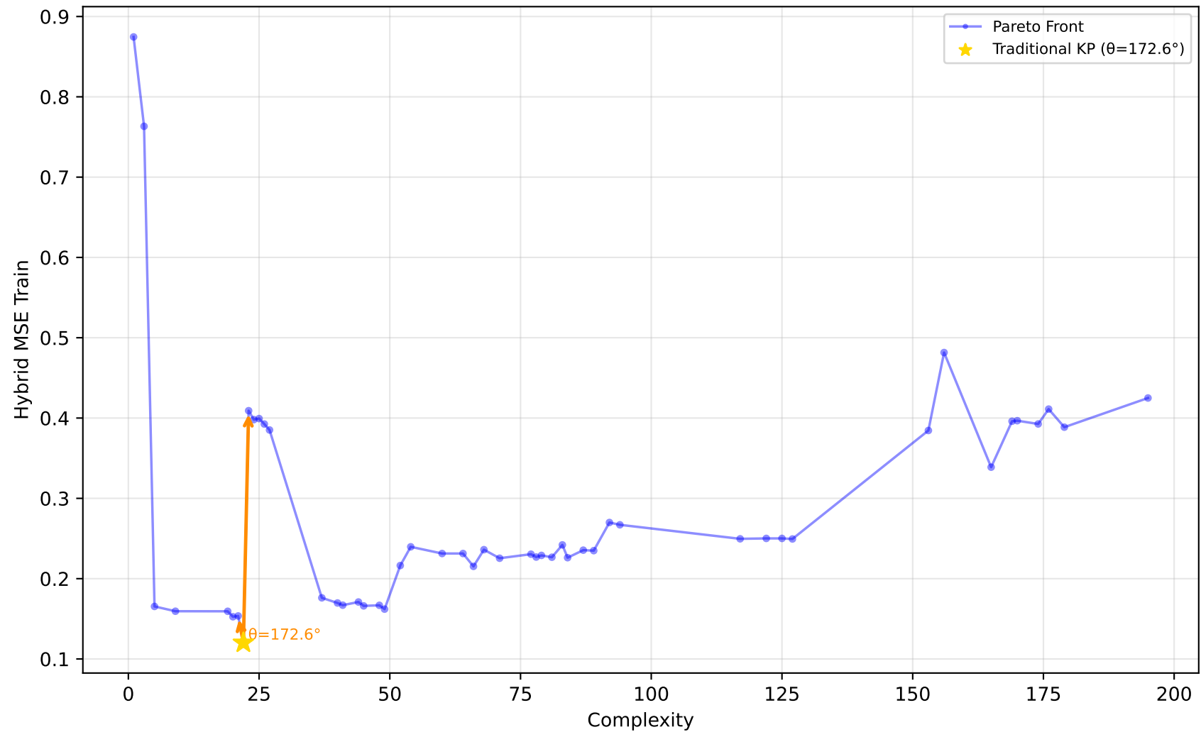
712_chscase_geyser1 - Run 2 - MVP - Hybrid MSE Train \lambda_1=0.20, \lambda_2=1.00, \lambda_3=1.00 | Difficulty: 1.00 | Method: hmr
