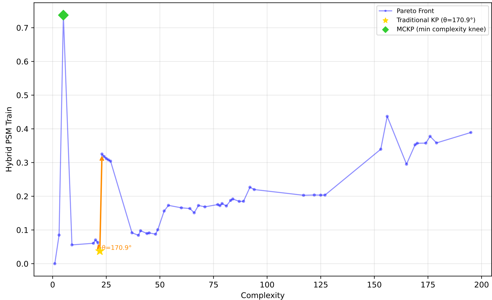
712_chscase_geyser1 - Run 2 - MVP - Hybrid PSM Train \lambda_1=0.20 , \lambda_2=1.00 , \lambda_3=1.00 | Difficulty: 1.00 | Method: hmr
