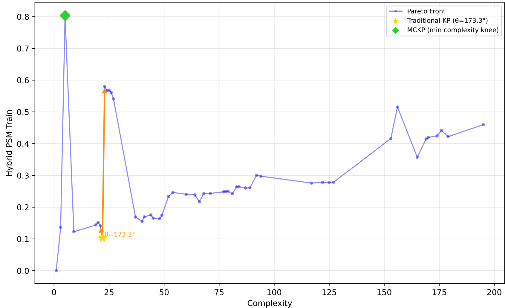
712_chscase_geyser1 - Run 2 - MVP - Hybrid PSM Train \lambda_1=1.00, \lambda_2=1.00, \lambda_3=1.00 | Difficulty: 1.00 | Method: hmr
