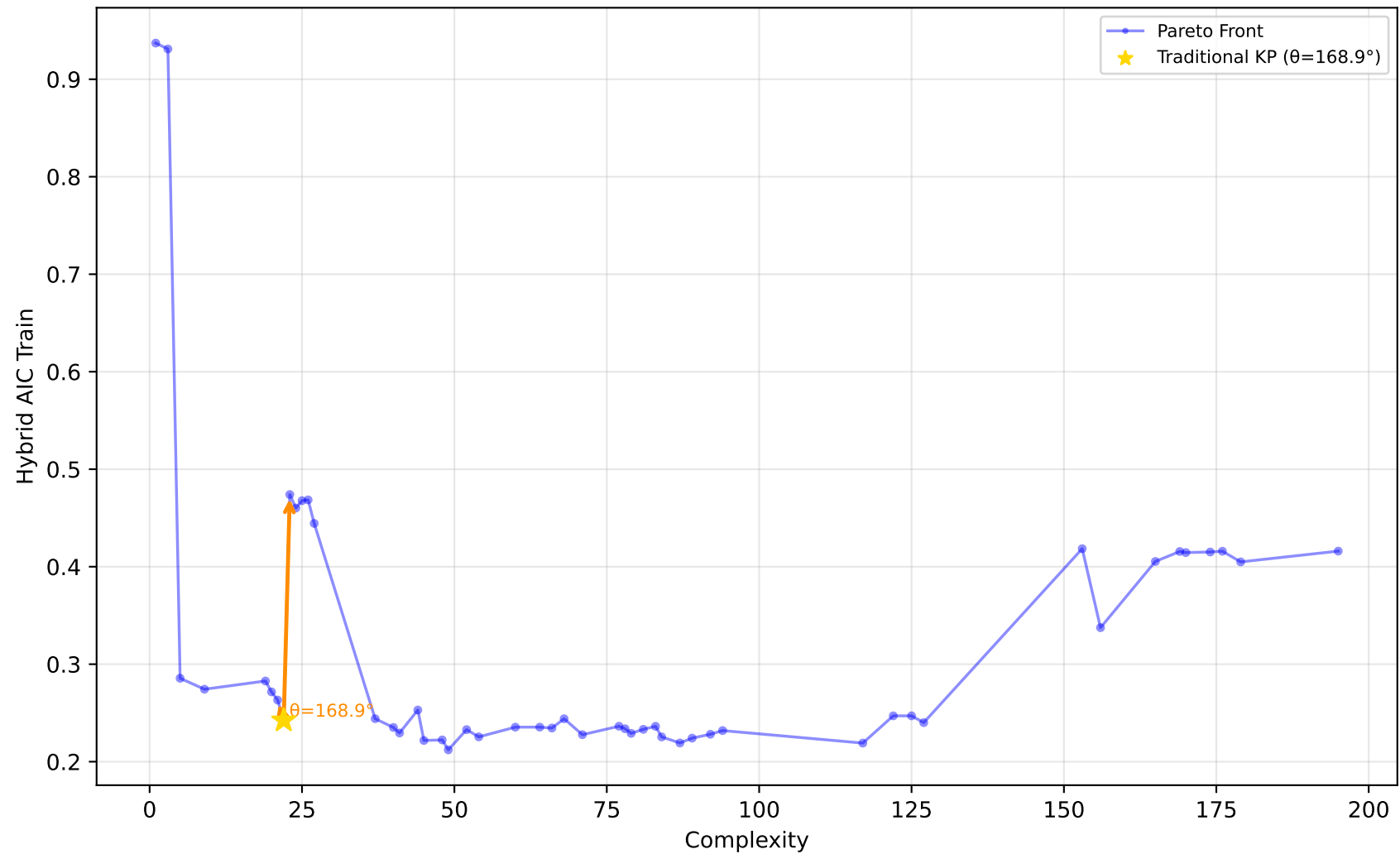
712_chscase_geyser1 - Run 2 - SVP - Hybrid AIC Train \lambda_1=1.00, \lambda_2=1.00, \lambda_3=0.00 | Difficulty: 1.00 | Method: hmr
